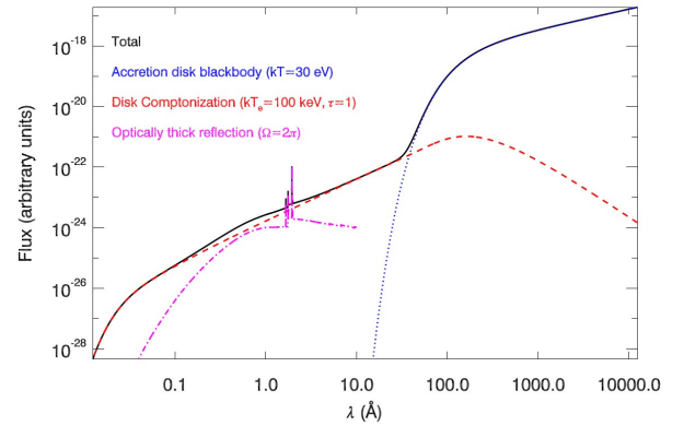
Figure 1: Schematic view of an AGN intrinsic UV-to-X-ray spectrum. Blue : thermal emission from a luminous accretion disk with a temperature at the innermost radius of 30 eV; red : unsaturated Comptonisation of soft disk photons with kT_e=100 keV and \tau_{es}=1 ; magenta : reflection from a plane-parallel infinite slab of cold ( \sim 10^4 K) matter (Compton continuum plus Fe and Nickel K_\alpha and K_\beta fluorescent emission lines; after Nandra et al. 2007)
