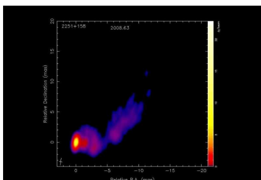
Figure 2: Figure 2: 3C454.3 shown at milliarcsecond scales for data taken from the MOJAVE VLBA campaign during the Bonning et al (2009) flare. A perusal of the time-dependent flare clearly shows that the jet launch from the core of the AGN is coincident with the double peaked flaring shown in the Bonning et al. results.
