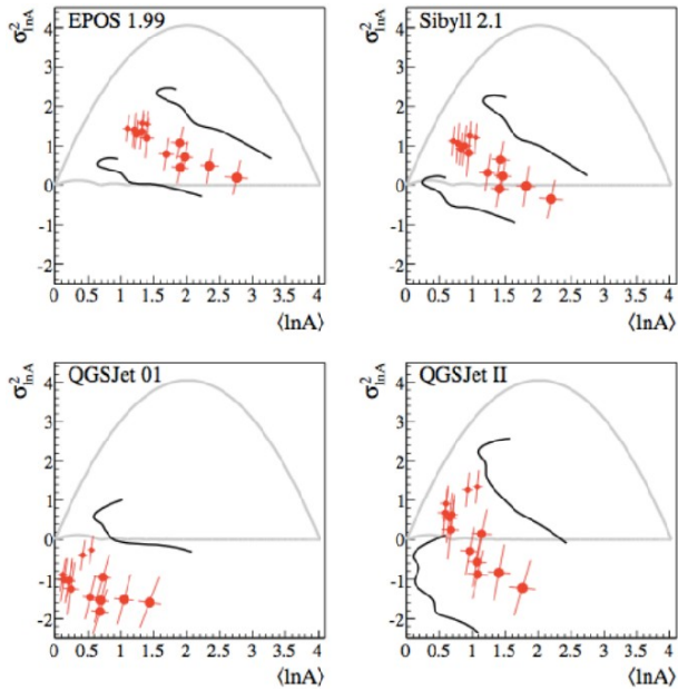
Figure 3: The Pierre Auger data in the (\langle \ln A \rangle, \sigma_{\ln A}^2) plane for different hadronic interaction models. Grey contours limit the allowed region, the systematic uncertainties are shown by the black lines.
