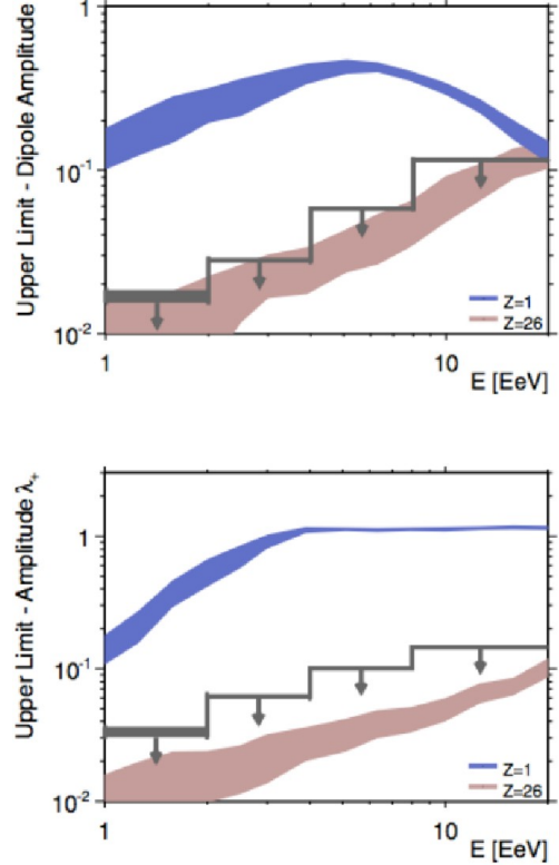
Figure 8: 99% CL upper limits on the dipole and quadrupole momenta as a function of energy.
