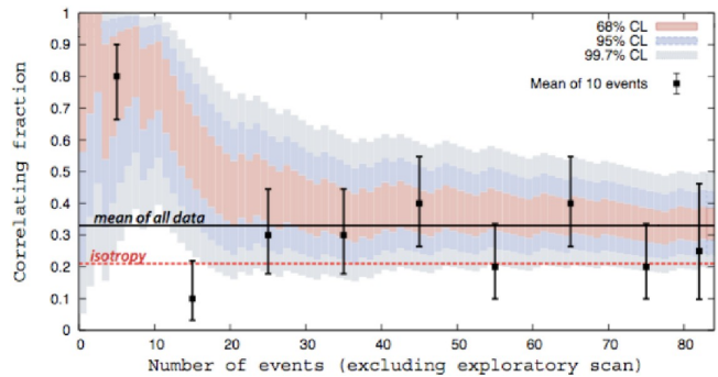
Figure 6: The correlating fraction as a function of the total number of time-ordered events. Different confidence levels are shown, together with the isotropy value p=0.21 and the current estimate of all data, p_{data} = 0.33 \pm 0.05 .
