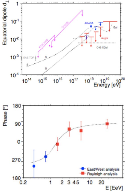
Figure 7: Equatorial dipole component (top) and phase of the first harmonic (bottom) as a function of energy.
