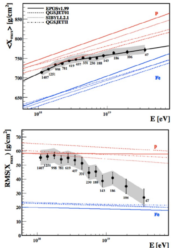
Figure 2: \langle X_{max} \rangle and RMS(X_{max}) as a function of energy, compared with the predictions of air shower simulations using different hadronic interaction models.
