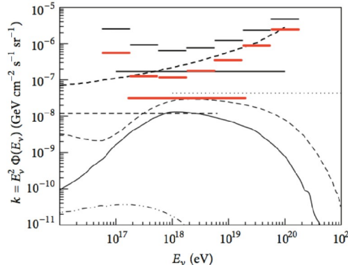
Figure 5: Differential and integrated upper limits on the single flavour E^{-2} \nu flux (thin black lines: downward-going \nu , thick red line: Earth-skimming \nu ). Different models are shown for comparison and discussed in [23]
