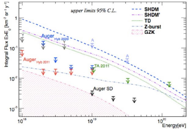
Figure 4: Upper limits on the integral photon flux. Different expectations are shown for comparison.
