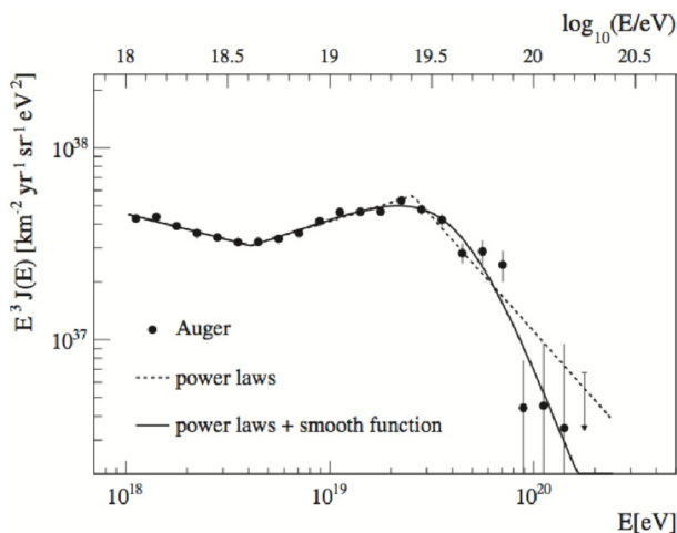
Figure 1: The combined Auger energy spectrum. Only statistical uncertainties are shown. The systematic uncertainty on the energy scale is 22%.
