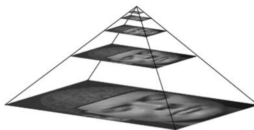
Fig. 1: The image I(\mathbf{x}) is embedded into a continuous family L(\mathbf{x}, \sigma) of gradually smoother versions of it. Hereby the original image corresponds to the scale \sigma = 0 [11]. Interest points are detected in this scale-space.
