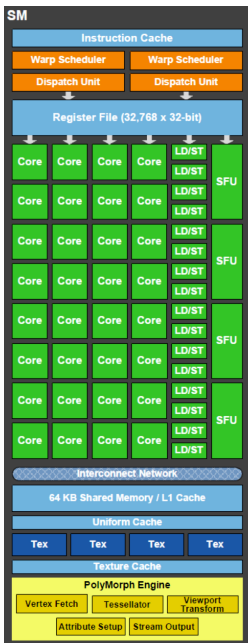
FIGURE 2. NVIDIA Fermi SMP [5].
