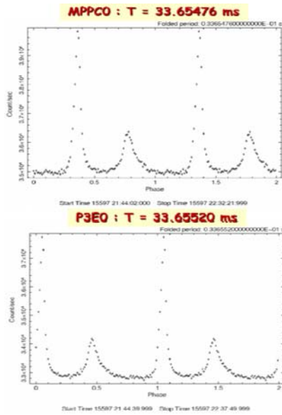
Fig. 6: Crab Pulsar light curves folded by “efold” for MPPC0 (upper) and P3E0 (lower)
