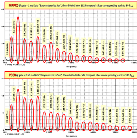
Fig. 5: Power Spectra of the Crab Pulsar signal detected by MPPC0 (upper) and P3E0 (lower)
