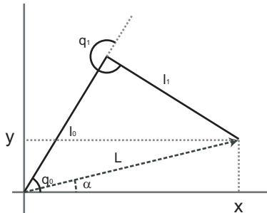
Fig. 2: A basic element as a main part for creating complex articulated structures
