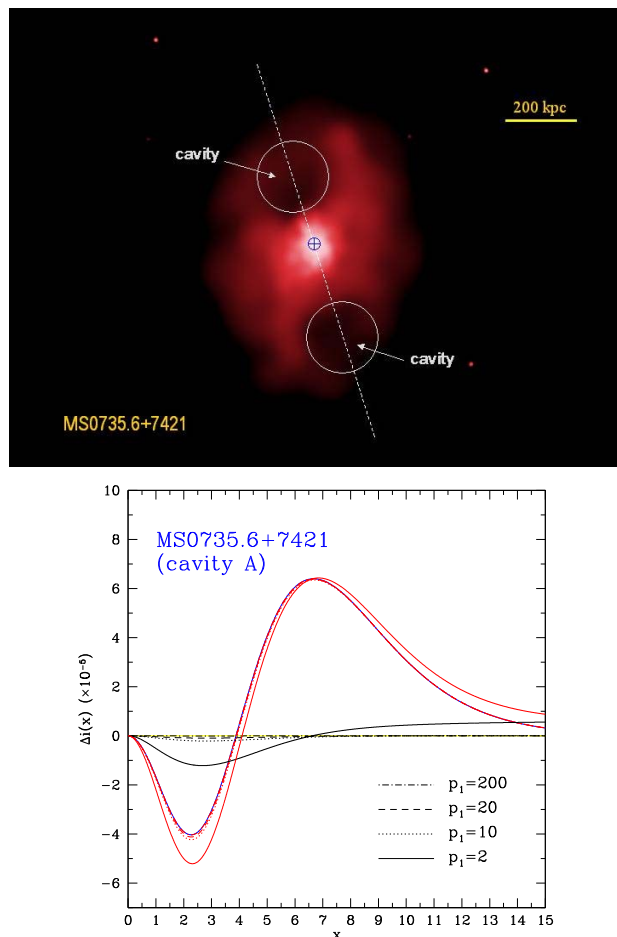
FIGURE 7. Top. The geometry of the cavities in the cluster MS0735.6+7421. Bottom. The SZE spectrum has been computed at a projected radius of \approx 125 kpc from the cluster center where the LOS passes through the center of northern cavity. The thermal SZE (blue), the non-thermal SZE from the cavity (black) and the total SZE (red) are shown. The non-thermal SZE is normalized to the cavity pressure P = 6 \times 10^{-11} erg cm ^{-3} , and is shown for various values of p_1 . Figure from [16].
