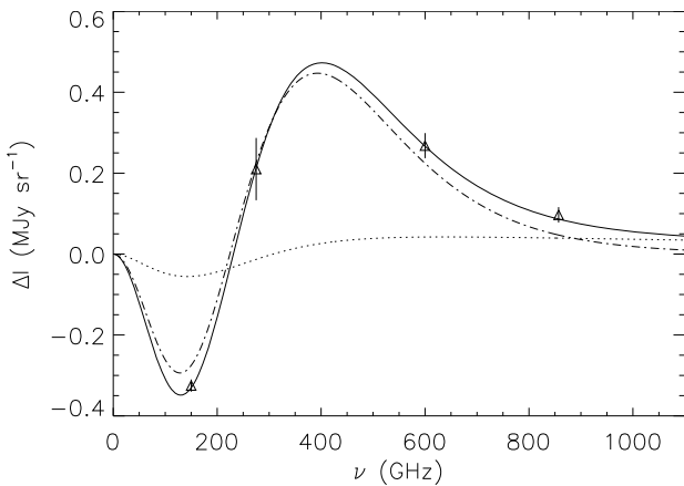
FIGURE 3. The SZE spectrum at the Bullet cluster center modeled with a thermal plus nonthermal plasma: thermal plasma with kT = 13.9 keV and \tau = 1.1 \times 10^{-2} (dot-dashed); nonthermal plasma with p_1 = 1 , s = 2.7 and \tau = 2.3 \times 10^{-4} (dotted); total SZE produced by the sum of the two plasmas (solid).
