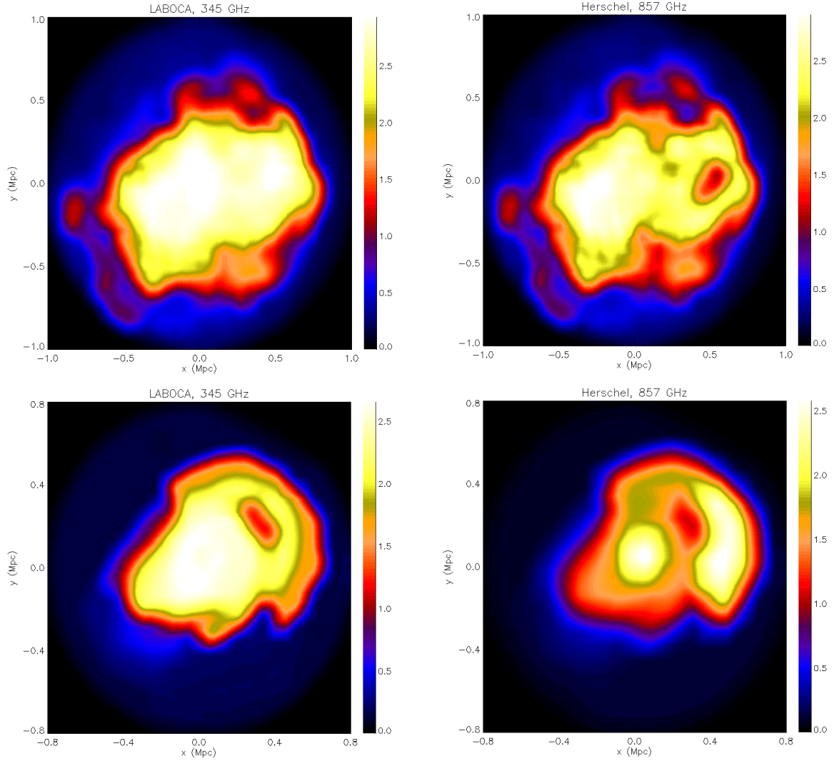
FIGURE 5. From top to bottom. The SZE signal to noise ratio map for the cluster 1E0657–558 at 345 GHz smoothed to the resolution of LABOCA and at 857 GHz smoothed to the resolution of Herschel-SPIRE. Analogous maps for the cluster A2219. Figures from [64].
