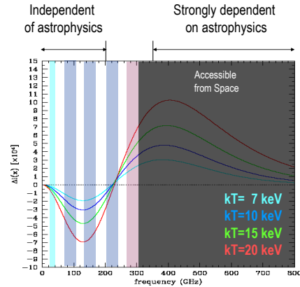
FIGURE 2. The thermal SZE spectrum of typical galaxy clusters for different plasma temperatures (as indicated) and the same value of the optical depth. The low- \nu part ( \nu \lesssim 220 GHz) of the spectrum depends mostly on the total Compton parameter y \propto \int dl P_{\text{tot}} and there is no strong spectral dependence on the temperature. The high- \nu part of the spectrum (at \gtrsim 300 GHz) shows a strong spectral dependence from the plasma temperature [23]. The usual frequency bands where the SZE is observed from the ground are shown as blue-cyan bands, while the region accessible only from space observations is shown by the gray shaded area.
