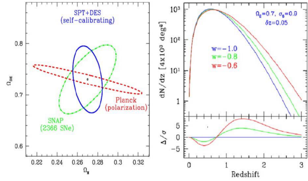
FIGURE 8. Left. Forecasts for the geometry constraints from the SPT+DES galaxy cluster survey, the SNAP SNe Ia mission, and Planck. Right. The expected redshift distribution (top) and quantified differences (bottom) for models where only the DE equation of state parameter w is varied. These models are normalized to produce the same local abundance of galaxy clusters. Figures from [50].
