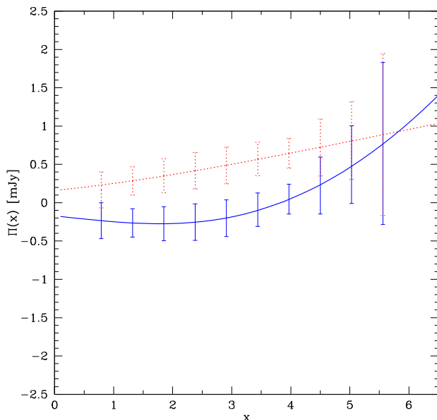
FIGURE 6. The thermal SZE polarization spectrum \Pi_{\text{th}} (blue solid) from a stacking analysis of 20 clusters with kT > 10 keV and \tau > 0.03 is compared with the same analysis for the kSZE polarization spectrum \Pi_{\text{k}} (red dotted). The statistical uncertainties refer to a stacking analysis produced with CORe [29].
