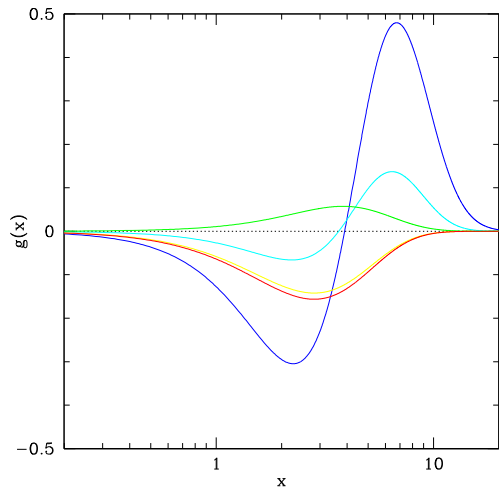
FIGURE 1. The SZE spectral shape g(x) is shown as a function of the nondimensional frequency x for different electronic populations residing in a cluster: thermal with k_B T_e = 8.2 keV (blue); warm with k_B T_e = 1 keV (cyan); secondary electrons from DM annihilation with M_\chi = 20 GeV (red); relativistic electrons which fit the Coma radio halo spectrum (yellow). The kinematic SZE with a negative peculiar velocity (green) is also shown for comparison. The amplitudes of the various curves have been artificially renormalized to highlight their frequency dependence.
