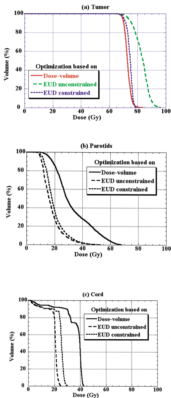
Figure 3. DVHs for the head and neck tumor shown in Figure 2. Solid lines corresponds to dose and dose-volume-based optimization, dashed lines correspond to unconstrained EUD-based optimization, dotted lines correspond to constrained EUD-based optimization: a) target DVHs, b) parotid glands DVHs, c) spinal cord DVH
