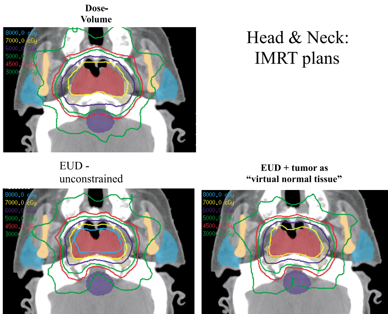
Figure 2. A color-wash display of dose distribution for a head and neck tumor for three planning approaches described in the text. The corresponding DVHs are shown in Figure 3.
