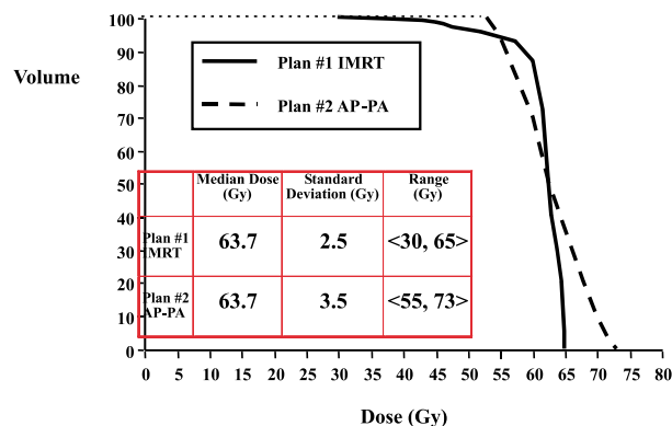
Figure 1. An example of dose-volume histograms for a target volume for IMRT dose delivery (Plan #1 – solid line) and for standard two parallel-opposed fields (Plan #2 – dashed line). A table shows the corresponding standard deviations of the target dose and the range of doses within the target volume.
