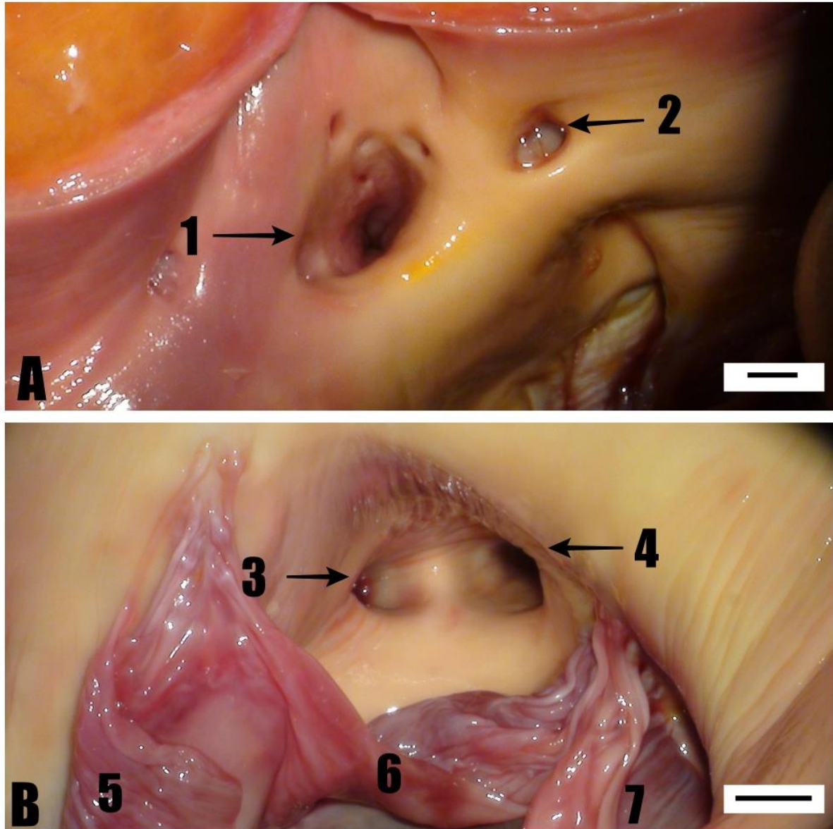
Figure 2. Overview of the aortic valve. A – additional coronary ostium in the left aortic sinus, B – lack of the main trunk of the left coronary artery. 1 – the left coronary ostium, 2 – the additional coronary ostium, 3 – the left circumflex branch, 4 – the paraconal interventricular branch, 5 – the septal semilunar leaflet, 6 – the left semilunar leaflet, 7 – the right semilunar leaflet. Scale bar 5 mm.
