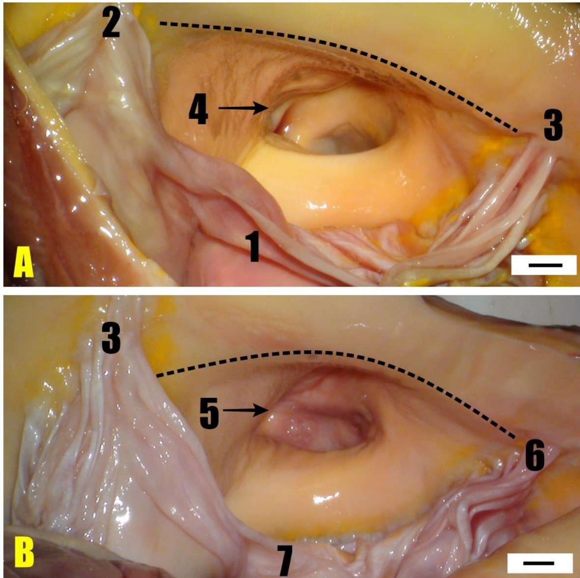
Figure 1. Location of the coronary ostia. A – the left coronary ostium, B – the right coronary ostium. The sinutubular junction (dotted lines). 1 – the left semilunar leaflet, 2 – the left aortic valve commissure, 3 – the intermediary aortic valve commissure, 4 – the left coronary ostium, 5 – the right coronary ostium, 6 – the right aortic valve commissure, 7 – the right semilunar leaflet. Scale bar 5 mm.
