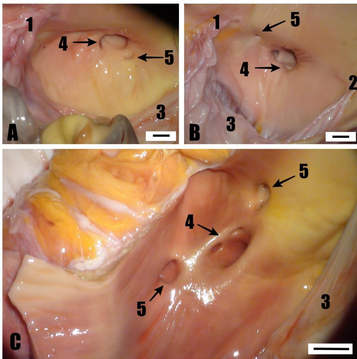
Figure 3. Overview of the aortic valve. A, B, C – the additional coronary ostia in the right aortic sinus. 1 – the intermediary aortic valve commissure, 2 – the right aortic valve commissure, 3 – the right semilunar leaflet, 4 – the right coronary ostium, 5 – the additional coronary ostium. Scale bar 5 mm
