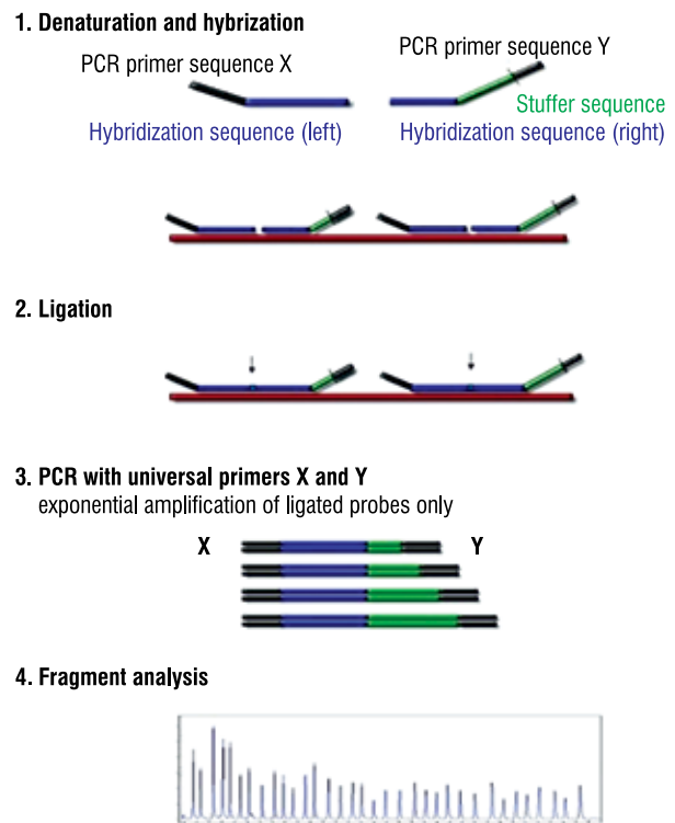
Figure 1. Schematic MLPA reaction. Sources: Company Website MRC Holland, http://www.mlpa.com/WebForms/WebFormMain.aspx?Tag=_wl2zCji-rCGANQgZPuTixsEyIW1MscfzuKj2NDFYc-g . Access: 05.05.2016
