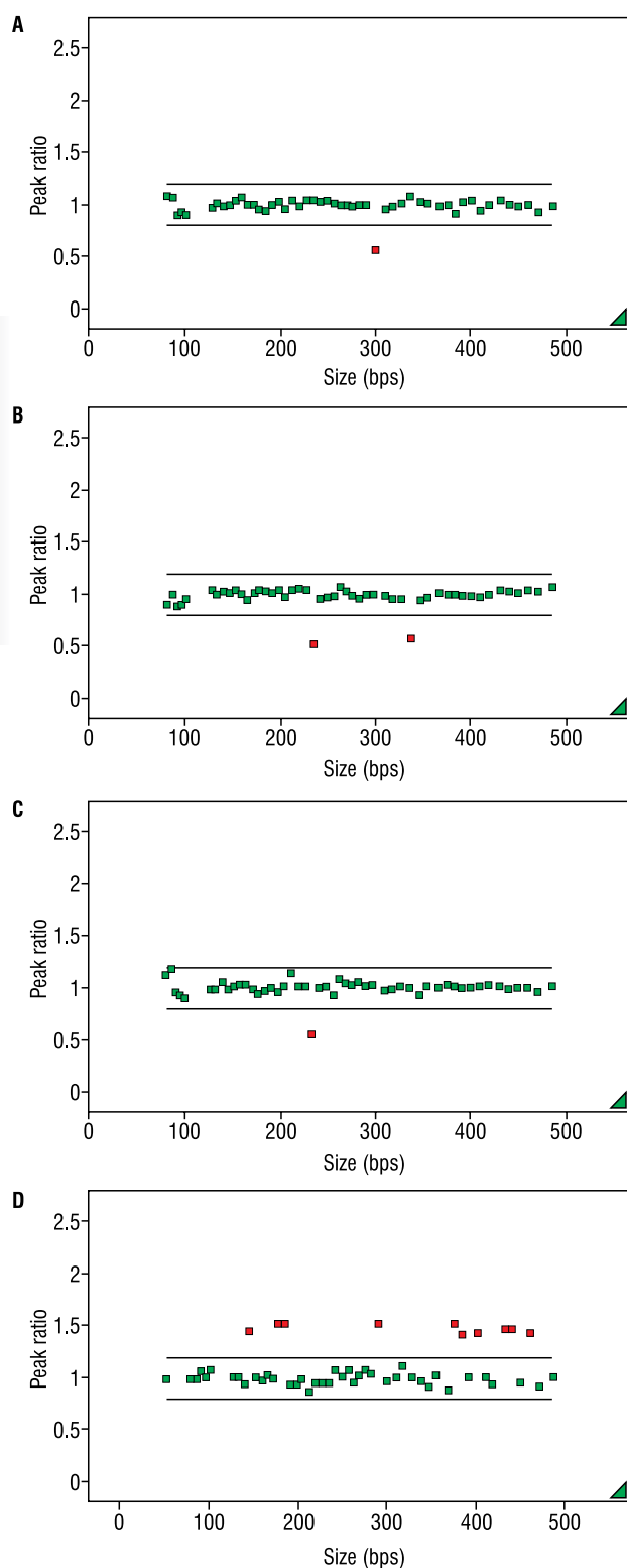
Figure 2. Selected results of MLPA reactions: A. Deletion in exon 4; B. Deletion in exons 5, 6a; C. Deletion in exon 6; D. Duplication in the Xp22.33-PAR1 regulatory region and in the CRLF2 and CSF2RA genes
