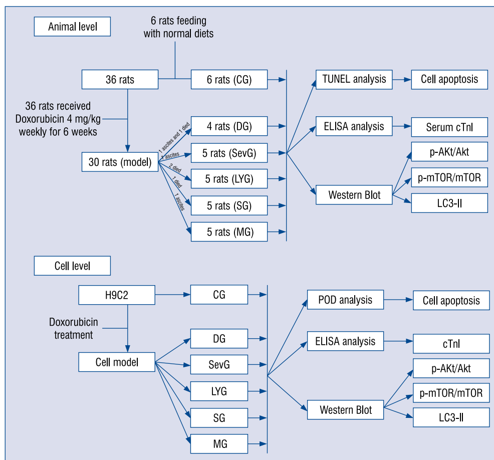
Figure 1. The flowchart of present study. Myocardial injury rat models were induced by doxorubicin and randomly divided into five groups according to different treatments: Doxorubicin group (DG), sevoflurane group (SevG), LY294002 group (Akt inhibitor, LYG), Solvent DMSO control group (SG) and autophagy inhibitor 3-methyladenine (3-MA) group (MG). Meanwhile, the healthy rats were assigned as a control group (CG). In SevG, the rats were inhaled with 2.4% sevoflurane for 2 h. In LYG, the rats were intraperitoneally injected with LY294002 0.3 mg/kg injection in 200- \mu L DMSO. In SG, the rats were intraperitoneally injected with the equal volume of DMSO. In MG, the rats were intraperitoneally injected with 3-MA at 30 mg/kg.
