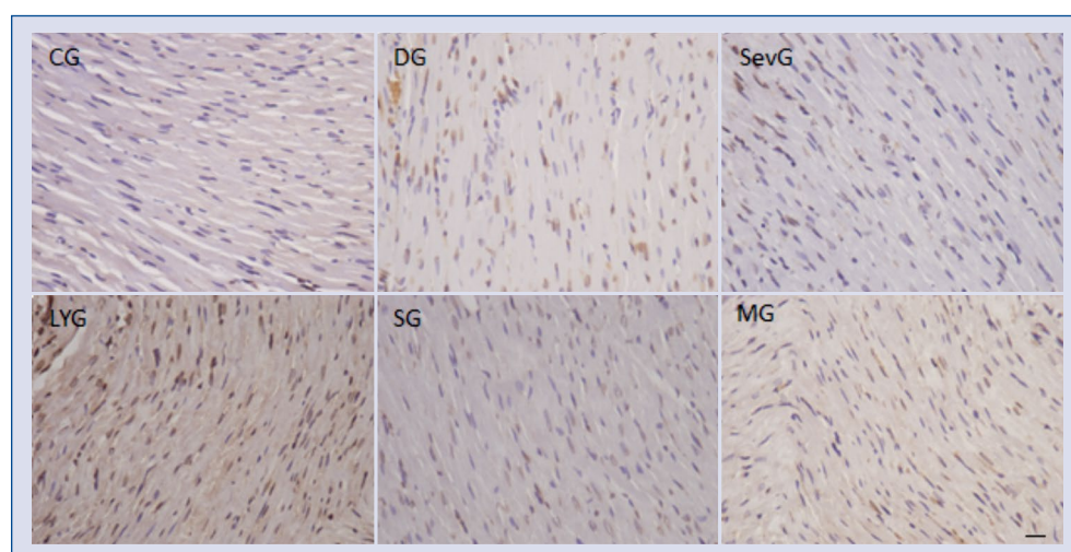
Figure 2. TUNEL analysis for myocardial cell apoptosis (400 \times ). Myocardial injury rat models were induced by doxorubicin and randomly divided into 5 groups according to different treatments: Doxorubicin group (DG), sevoflurane group (SevG), LY294002 group (Akt inhibitor, LYG), Solvent DMSO control group (SG) and autophagy inhibitor 3-methyladenine (3-MA) group (MG). Meanwhile, the healthy rats were assigned as a control group (CG). In SevG, the rats were inhaled with 2.4% sevoflurane for 2 h. In LYG, the rats were intraperitoneally injected with LY294002 0.3 mg/kg injection in 200- \mu L DMSO. In SG, the rats were intraperitoneally injected with 200- \mu L DMSO. In MG, the rats were intraperitoneally injected with mg/kg 3-MA in 200- \mu L DMSO. 1 bar = 10 \mu m.
