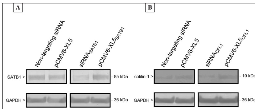
Figure 1. Post-translational expression of SATB1 and cofilin-1 in the MCF-7 cells. A. Post-translational expression of SATB1 in the cells transfected with siRNA against SATB1 or pCMV6-XL5 expression plasmid with cloned cDNA of SATB1; B. Post-translational expression of cofilin-1 in the cells transfected with siRNA against cofilin-1 or pCMV6-XL5 expression plasmid with cloned cDNA of cofilin-1
