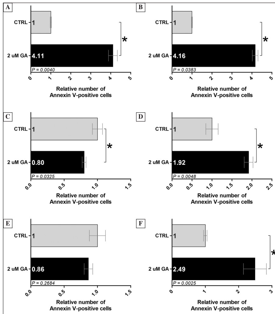
Figure 2. Relative number of the Annexin V-positive MCF-7 cells after the 24 h treatment with 2 \mu\text{M} geldanamycin. A. Cells transfected with non-targeting siRNA; B. Cells transfected with pCMV6-XL5 empty plasmid; C. Cells transfected with siRNA against SATB1; D. Cells transfected with pCMV6-XL5 expression plasmid with cloned cDNA of SATB1; E. Cells transfected with siRNA against cofilin-1; F. Cells transfected with pCMV6-XL5 expression plasmid with cloned cDNA of cofilin-1. Data are expressed as the ratio of the percentage of Annexin V-positive cells after exposition to 2 \mu\text{M} GA to the percentage of Annexin V-positive control cells
