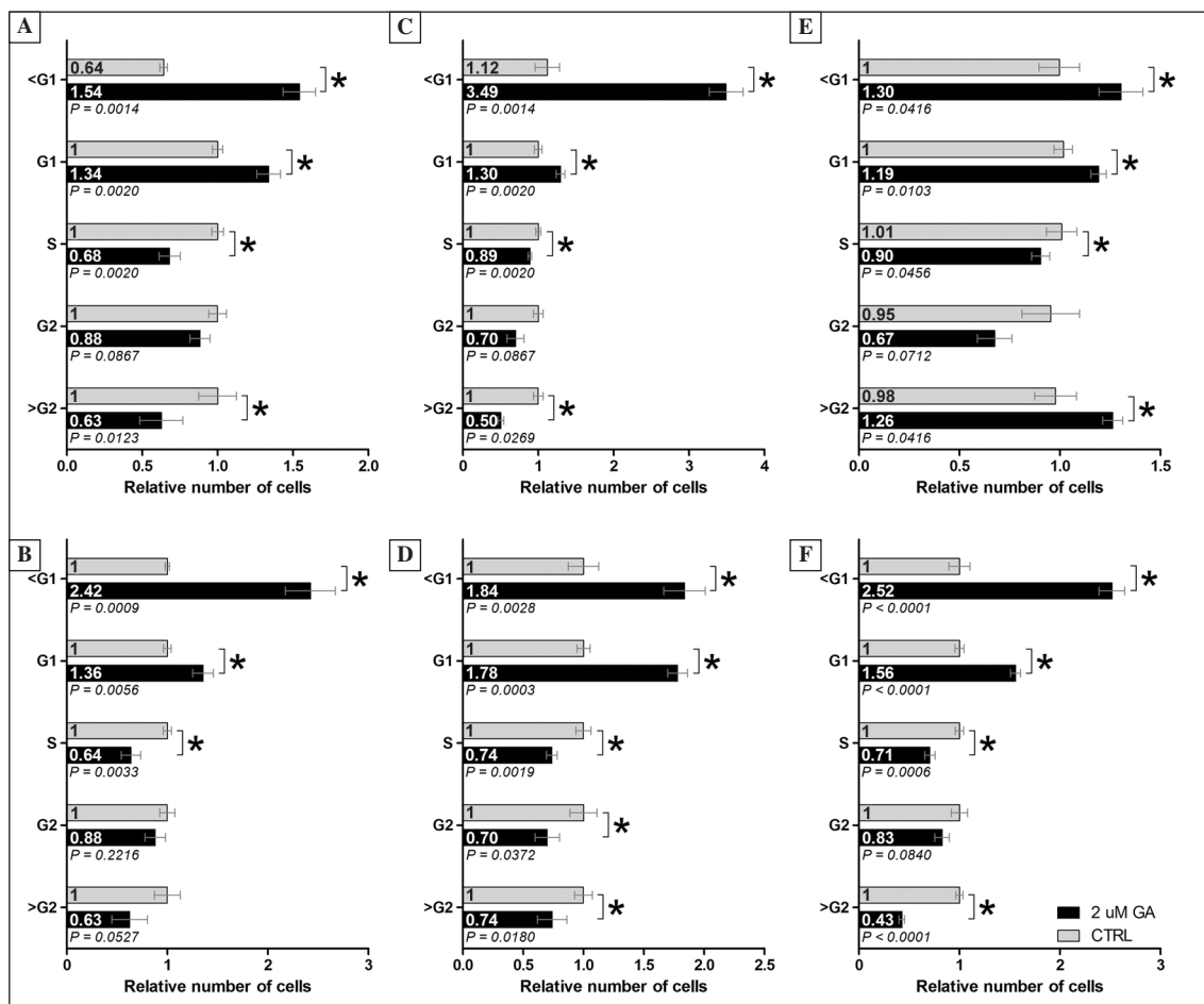
Figure 3. Relative number of the MCF-7 cells in particular phases of cell cycle after the 24 h treatment with 2 μM geldanamycin. A. Cells transfected with non-targeting siRNA; B. Cells transfected with pCMV6-XL5 empty plasmid; C. Cells transfected with siRNA against SATB1; D. Cells transfected with pCMV6-XL5 expression plasmid with cloned cDNA of SATB1; E. Cells transfected with siRNA against cofilin-1; F. Cells transfected with pCMV6-XL5 expression plasmid with cloned cDNA of cofilin-1. Data are expressed as the ratio of the percentage of cells in appropriate phase of the cell cycle after exposition to 2 μM GA to the percentage of control cells in the same phase of the cell cycle
