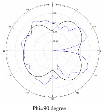
Figure 14: Comparison of the simulated radiation patterns of the proposed antenna with (blue dashed line) and without (black solid line) connecting to the laptop computer at 5 GHz band
