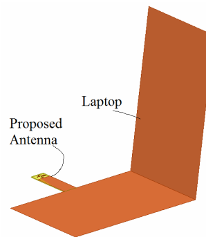
Figure 10: Simulation model of the USB dongle connecting to the laptop computer in HFSS
