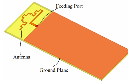
Figure 1: Proposed ILA based on the fractal geometry
