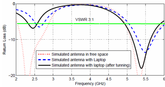
Figure 11: Simulated return loss of the proposed antenna with and without the laptop
