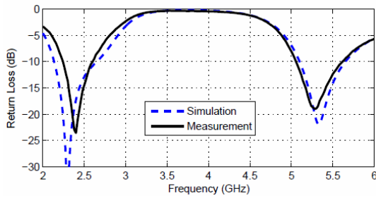
Figure 5: Comparison of the simulated and measured return loss of the fractal ILA
