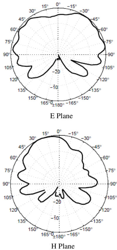
Figure 6: Measured radiation patterns of the printed multiband ILA antenna at 2.4GHz
