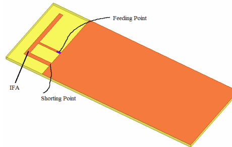
Figure 7: The structure of a typical Inverted-F antenna
