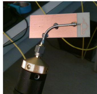
Figure 4: Photo of the fabricated prototype during return loss measurement
