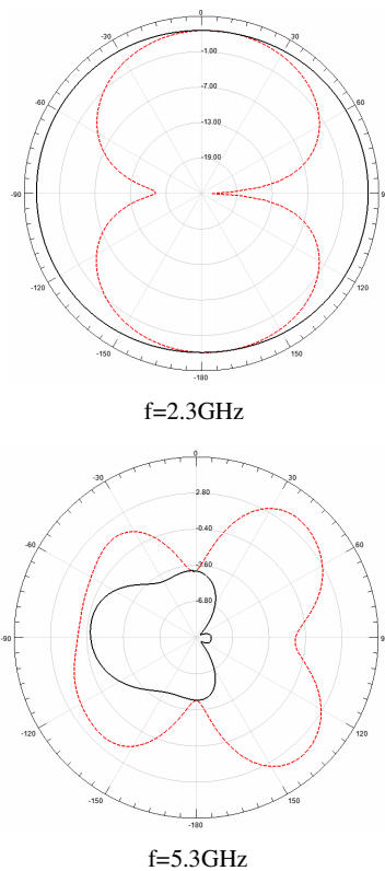
Figure 9: The simulated radiation patterns of the proposed antenna in free space ( \Phi=0 degree: dashed line; \Phi=90 degree: solid line)
