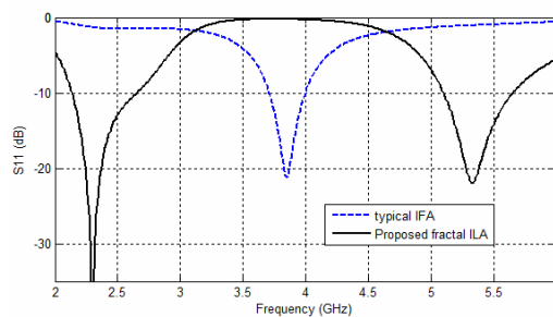
Figure 8: Comparison of the simulated return loss between the proposed fractal ILA and a typical Inverted-F antenna
