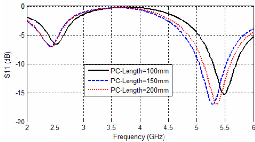
Figure 12: Simulated return loss of the proposed antenna with laptop computer of different length
