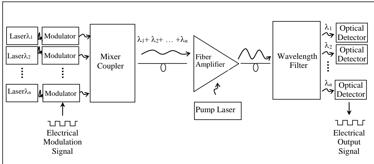
Fig 1. Typical wavelength-division multiplexing-fiber optic communication system.
