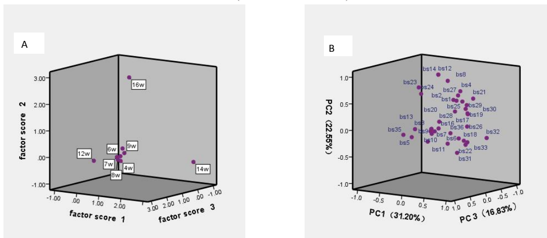
FIGURE 2 Principle component analysis of volatile compounds of grape skin. A. PCA score plot. B. Loading plot of components 1, 2 and 3. Note: “bs” refers to volatiles in grape skins. For details, refer to the Table 1.
