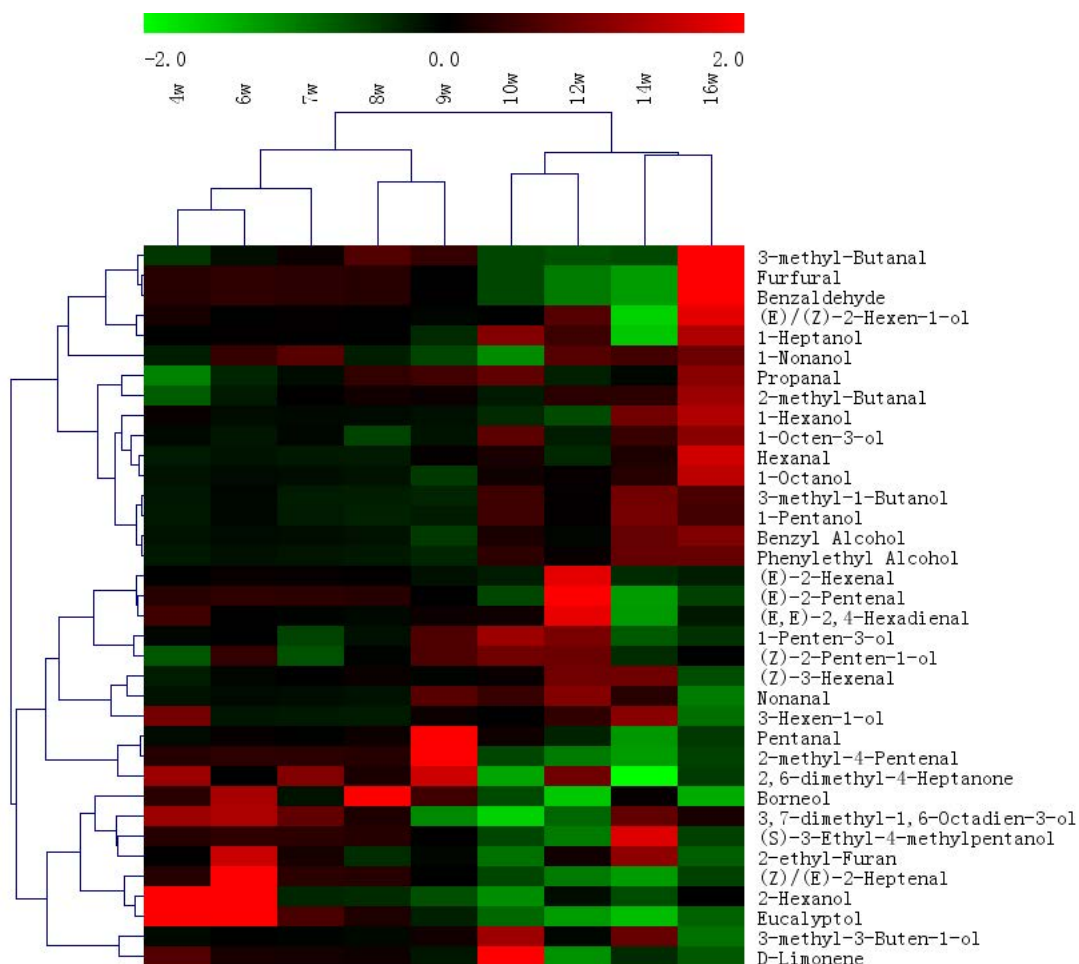
FIGURE 1 Heatmap of the concentration of volatiles in grape skin. Note: W (weeks after anthesis)
