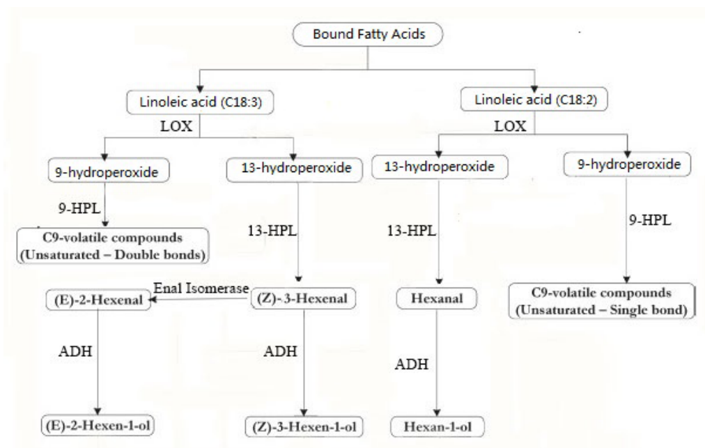
FIGURE 1S Schematic drawing of the GLV pathway in plants
