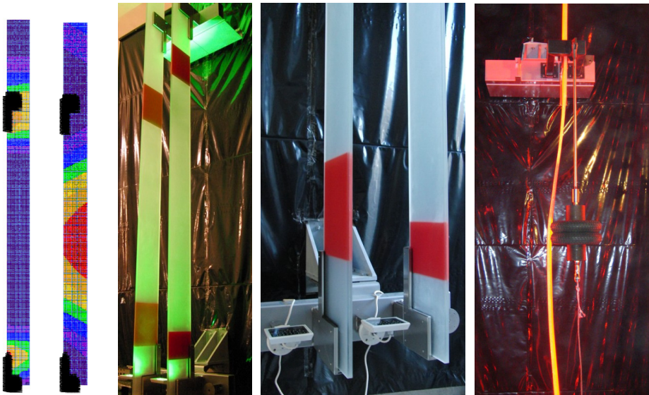
Figures 5-9 (from left to right): Stress analysis, Deflection analysis, Visual mock up © Bellpart, Impact testing stage 3 © Bellpart
