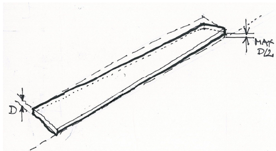
Figure 4: Tolerances for warp of fin
