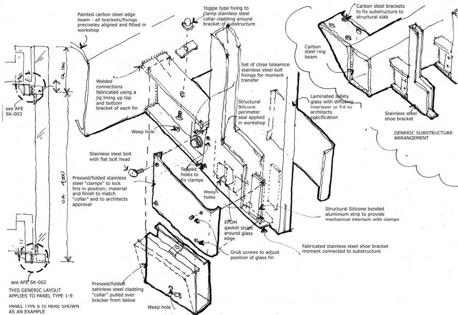
Figure 10: Design Sketch showing bottom bracket arrangement
