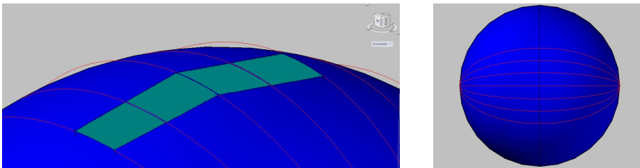
Figure 2: Study of geometry. Approximation of sphere with cylindrical elements
