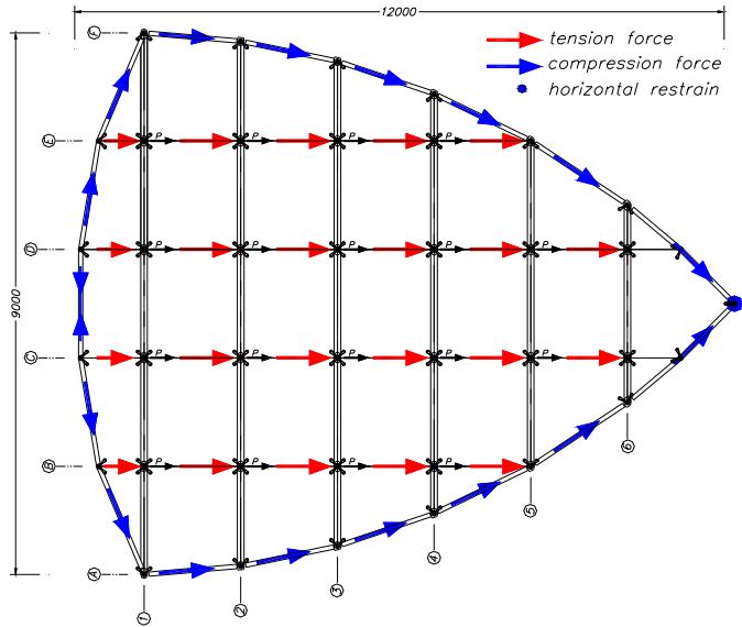
Figure 5: Horizontal load path.
