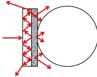
Fig. 3 Radiation laterally shifted after incidence on a light-scattering coating on an otherwise transparent glass pane. In the case where the incident beam is narrow and the aperture is too small, only a fraction of the transmitted radiation will enter the integrating sphere.
