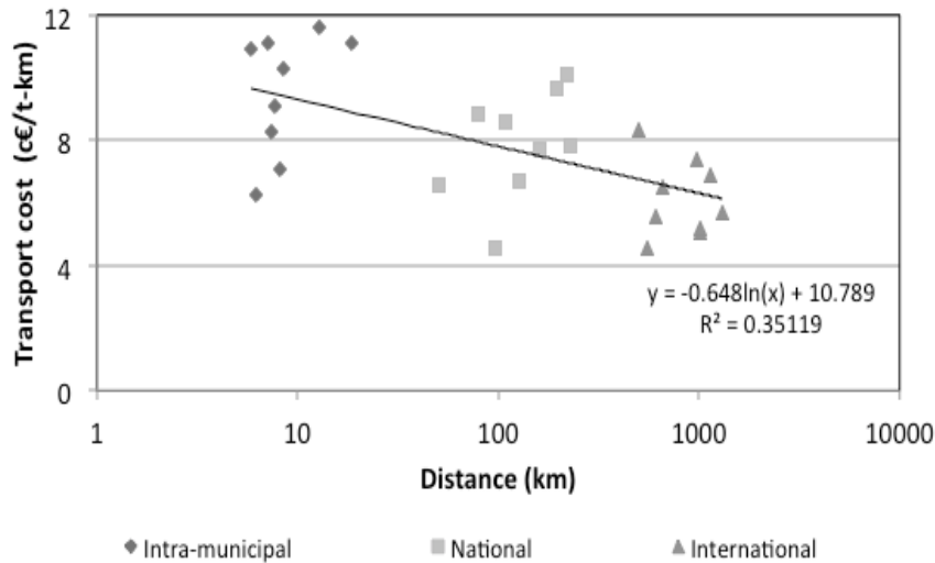
Figure 6. Operation cost and average transport distance on a logarithmic scale for Spain (2006). Notes: the transport cost (X) elasticity regarding the average transport distance (Y) is calculated by the following expression \eta_{x,y} = \partial Y / \partial X * X / Y = -0.648 / Y ; the linear fit reported the square correlation coefficient, the slope, and the intercept. Source: MFO, 2009; and this study.
