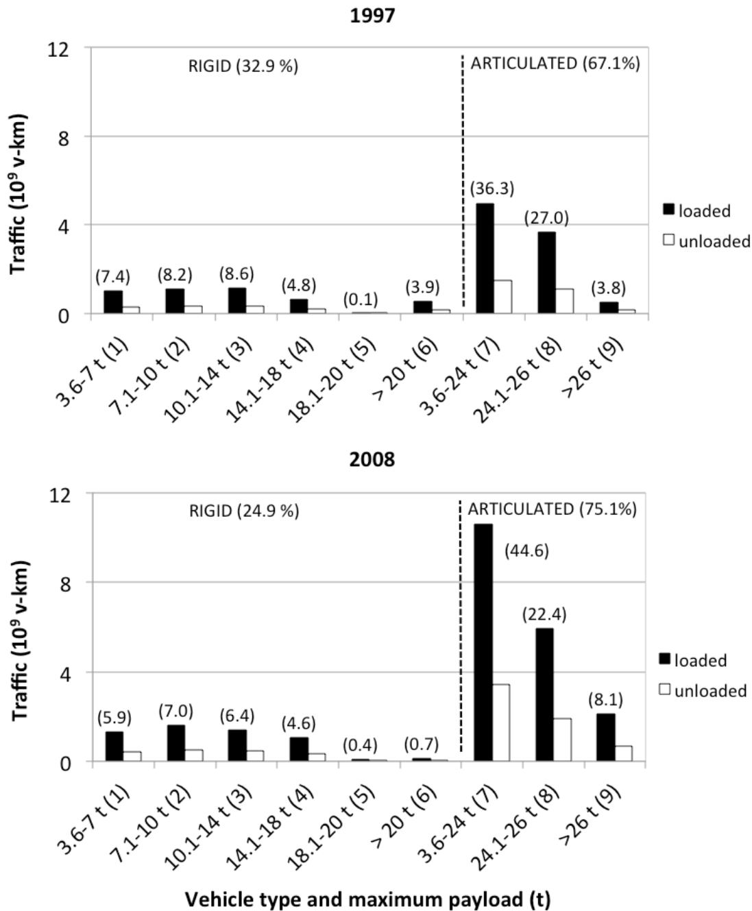
Figure 1. Distribution of v-km by type of vehicle and payload. Note: traffic shares of laden kilometres in brackets; 1 equivalent to <10 t Gross Vehicle Weight (GVW); 2 10-13.5 t; 3 14.1-18 t; 4 18-24 t; 5 24.1-26 t; 6 >26 t; 7 10-32 t (GVW); 8 32.1-38 t; 9 38.1-44 t; Source: (MFO, 2010).
