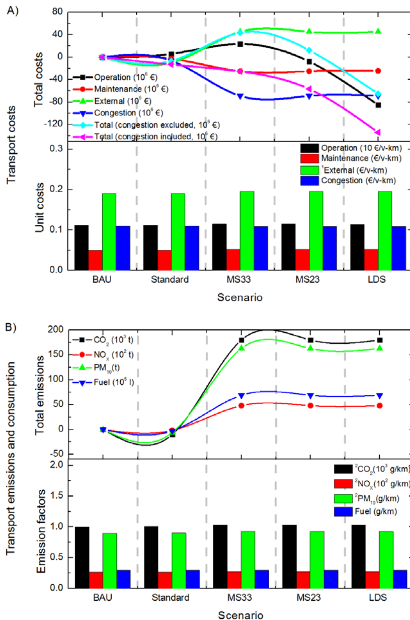
Figure 4. Road freight transport costs and emissions. A) Operation, maintenance, external, and congestion cost balances of the aggregated freight road transport according to substitution scenarios (10 6 €, 2008 constant prices). B) CO 2 (10 3 t), NO x (10 2 t), PM 10 (t) emissions and fuel consumption (10 6 l).
