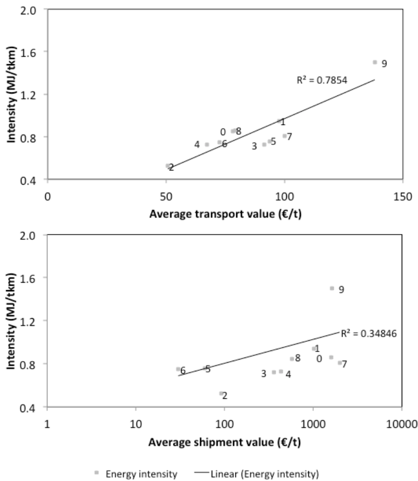
Figure 7. Energy intensity of road transport operations in Spain, average operation transport cost (€/t, upper graph), and average value of the shipment on a logarithmic scale (€/t, lower graph), 2006. The linear fits reported the square correlation coefficients. Source: MFO, 2009; and this study.
