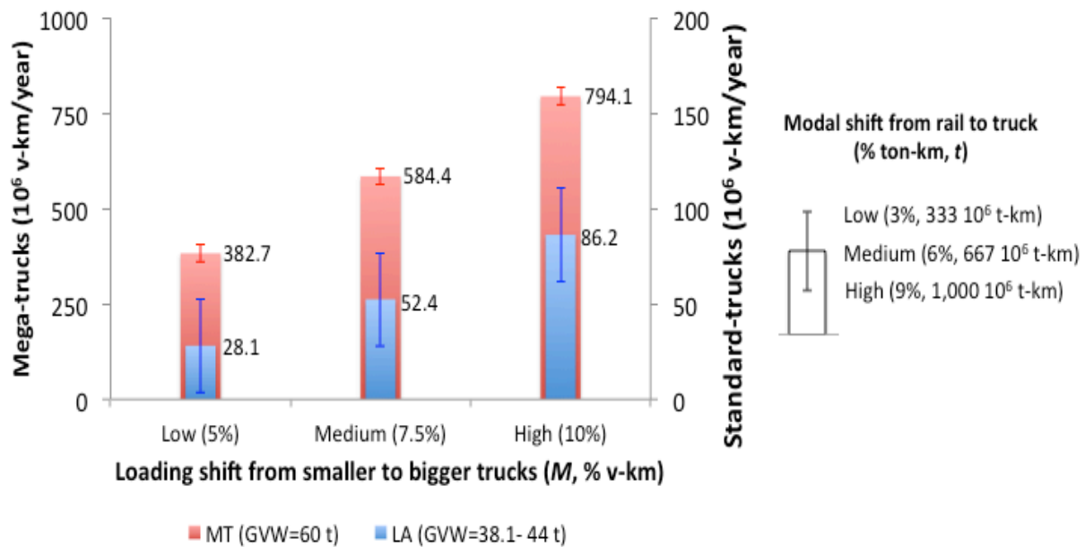
Figure 3. Estimates of vehicle kilometre reductions, resulting from the increase in the maximum allowable gross weight of trucks (in million v-km per year), by loading and modal shifts.
