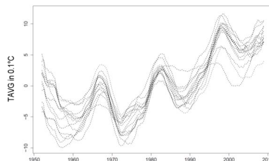
Figure 3. Estimated individual TAVG trends of all Scandinavian stations recording prior to 1952 and expressed in mean-deviation units.
