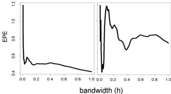
Figure 2. Exemplary EPE-function for GCV. Left: Epanechnikov's kernel. Right: IMSE-optimal boundary kernel of first order.
