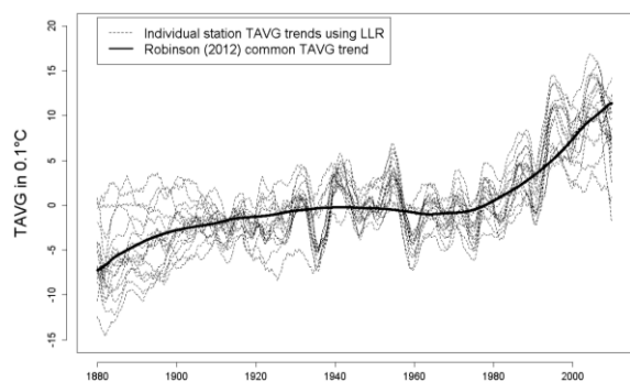
Figure 4. Common European trend in TAVG using Robinson (2012), GCV, the NWE, and an IMSE-optimal boundary kernel of first order.
