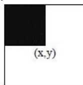
Gambar 7. Integral Image
