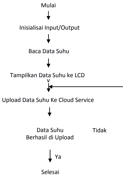
Gambar 4. Flowchart
