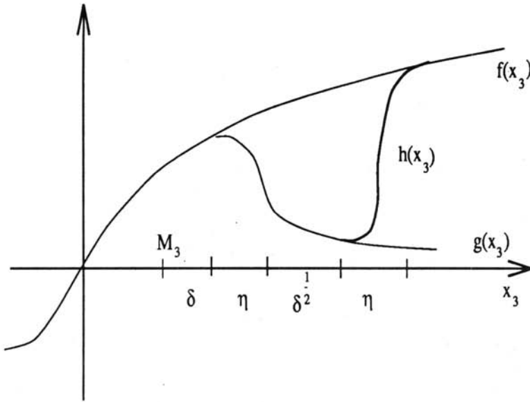
Figure 3: Function h(x) .
