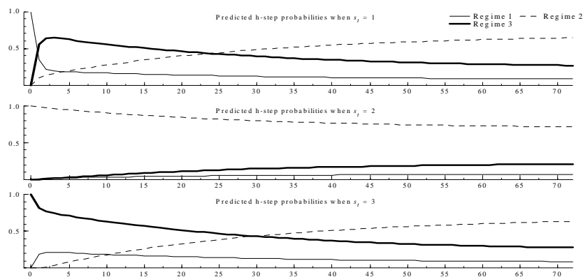
GRAPH 2 - CONDITIONAL DURATION'S PROBABILITIES - MS(3)AR(5)-d1
