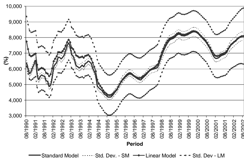
GRAPH 5 - COMPARISON OF ESTIMATES - CONVEX AND LINEAR NAIRU
