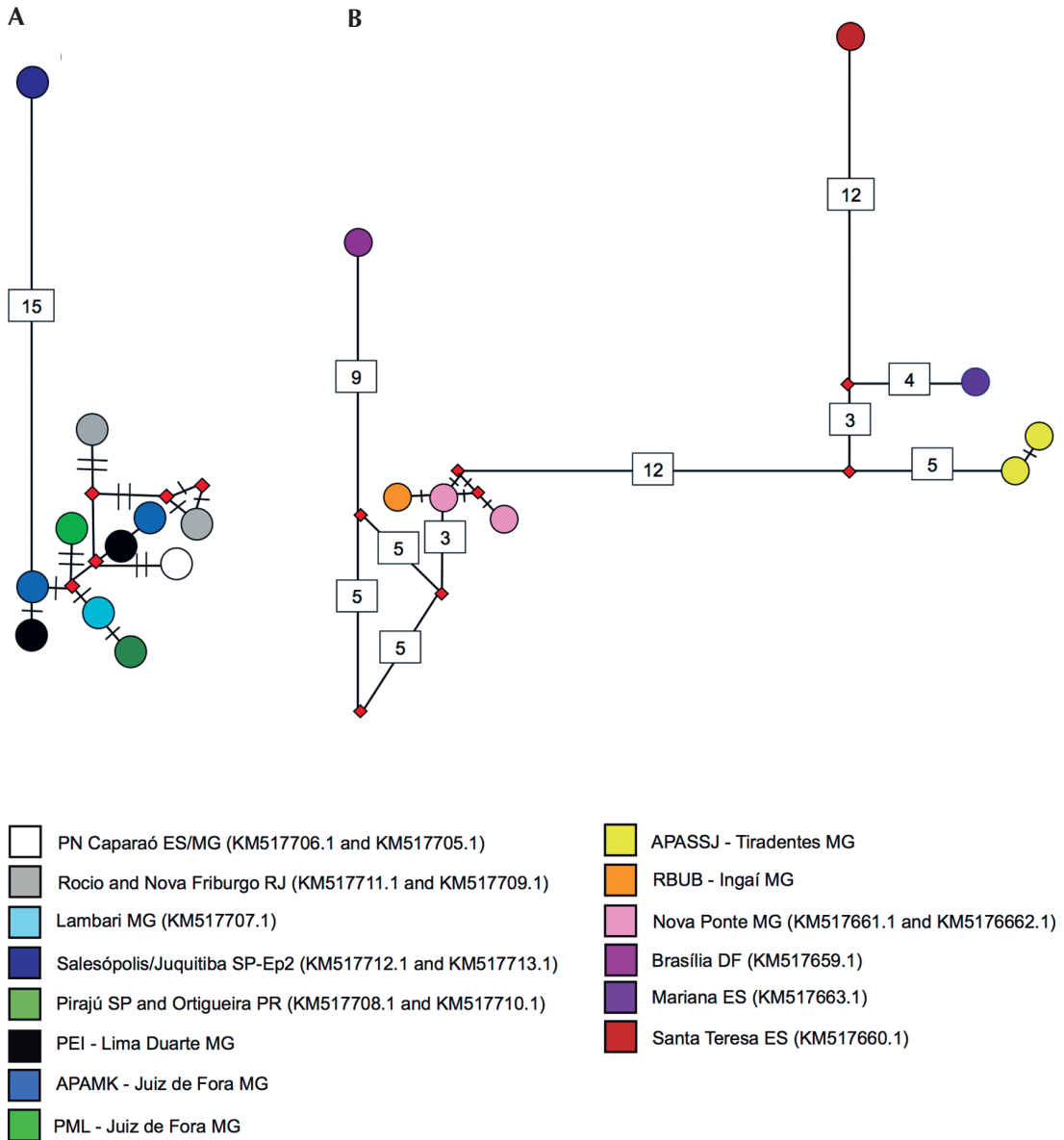
Figure 3. MJ networks describing the relationship among the Enyalius mtDNA haplotypes (234-bp). The relationship among the 11 haplotypes of E. perditus is shown on the left ( A ), and that of the eight haplotypes of E. bilineatus is on the right ( B ; this study and Rodrigues et al. [2014]). The median vectors are represented by the red diamonds. The values inside the squares are the mutational points. The sizes of the circles size do not reflect the frequencies of samples from each haplotype.
