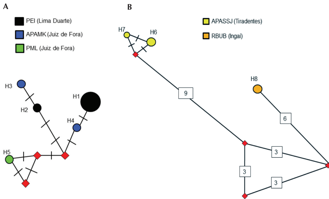
Figure 2. MJ networks describing the relationship among the Enyalilus mtDNA haplotypes (234-bp). The relationship among the five haplotypes of E. perditus is shown on the left (A), that of the haplotypes of E. bilineatus is on the right (B). H1 to H8 represents the Haplotypes 1–8. The median vectors are represented by the red diamonds. The values inside the squares are mutational points. The sizes of the circles size represent the frequencies of each haplotype.
