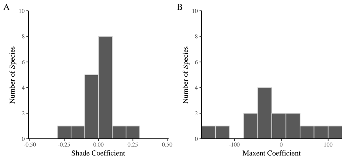
Figure 4. Histograms of effect sizes for species with greater than three observations that: had shade as a predictor in their best models ( n = 17 )(A) and species' that had Maxent as a predictor in their best models ( n = 15 )(B).
