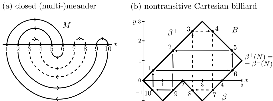
FIGURE 1.5. (a) The simple closed meander M of 1.3(a). (b) A nontransitive billiard B with boundaries \beta^\pm , N = 5 and associated meander M = \Phi(B) . Horizontal/vertical flights at half-integer y/x in B again correspond to the n = 5 upper/lower arches in M , respectively. One flight path/meander component is distinguished by dashing.
