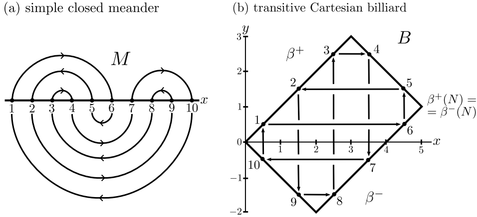
FIGURE 1.4. (a) The simple closed meander M of figure 1.2(a). (b) A transitive billiard B with boundaries \beta^\pm , N = 5 , and associated meander M = \Phi(B) . Note how horizontal flights at half-integer constant y in B correspond to the N = 5 upper arches in M , and vertical flights at half-integer constant x correspond to the N = 5 lower rainbow arches.
