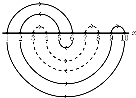
FIGURE 1.3. (a) A closed rainbow (multi-) meander with two connected components; one distinguished by dashed arches. (b) A corresponding nontransitive plane Cartesian billiard; one flight path distinguished by dashed lines.
