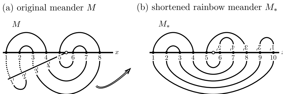
FIGURE 5.6. (a) The original closed circle-free meander M with N = 4 of figure 5.5(a), slightly opened at intersections 1, \dots, N_* = 5 < 2N . Note the lower rightmost innermost arch at (N_*, N_* + 1) . (b) The fully opened rainbow meander M_* with N_* < 2N upper arches and 2N_* < 4N intersections.
