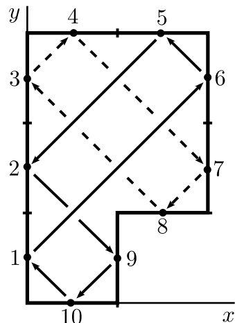
FIGURE 1.3. (a) A closed rainbow (multi-) meander with two connected components; one distinguished by dashed arches. (b) A corresponding nontransitive plane Cartesian billiard; one flight path distinguished by dashed lines.
