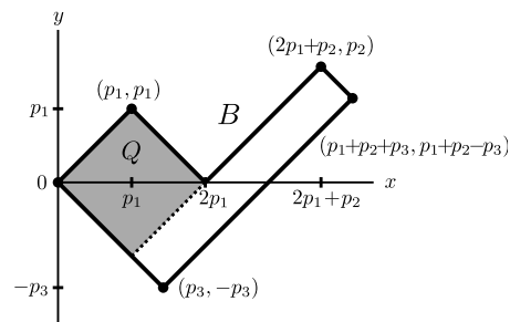
FIGURE 6.3. Circle-free rainbow meander M = M(p_1, p_2, p_3) with p_1 < p_3 , in (a), and corresponding L-shaped billiard B = B(p_1, p_2, p_3) , in (b). Note the shaded p_1 \times p_1 square Q in the left wing of B with the dashed line as boundary.
