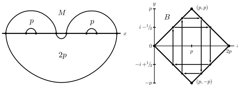
FIGURE 6.1. (a) Symmetrically cleaved rainbow meander M = M(p, p) . (b) Corresponding square billiard B = B(p, p) with p closed rectangular billiard paths.
