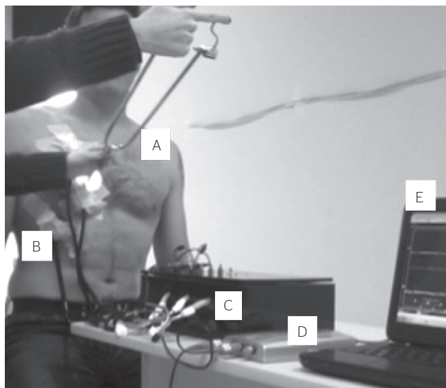
Figure 2. Illustrative image of the experimental design. (A) Application of Diottix®; (B) stethoscopes placed in the anterior region of the right hemithorax; (C) connected to the electret microphone; (D) connected to the oscilloscope and (E) interfaced with the software to analyze the amplitude and frequency of signals
