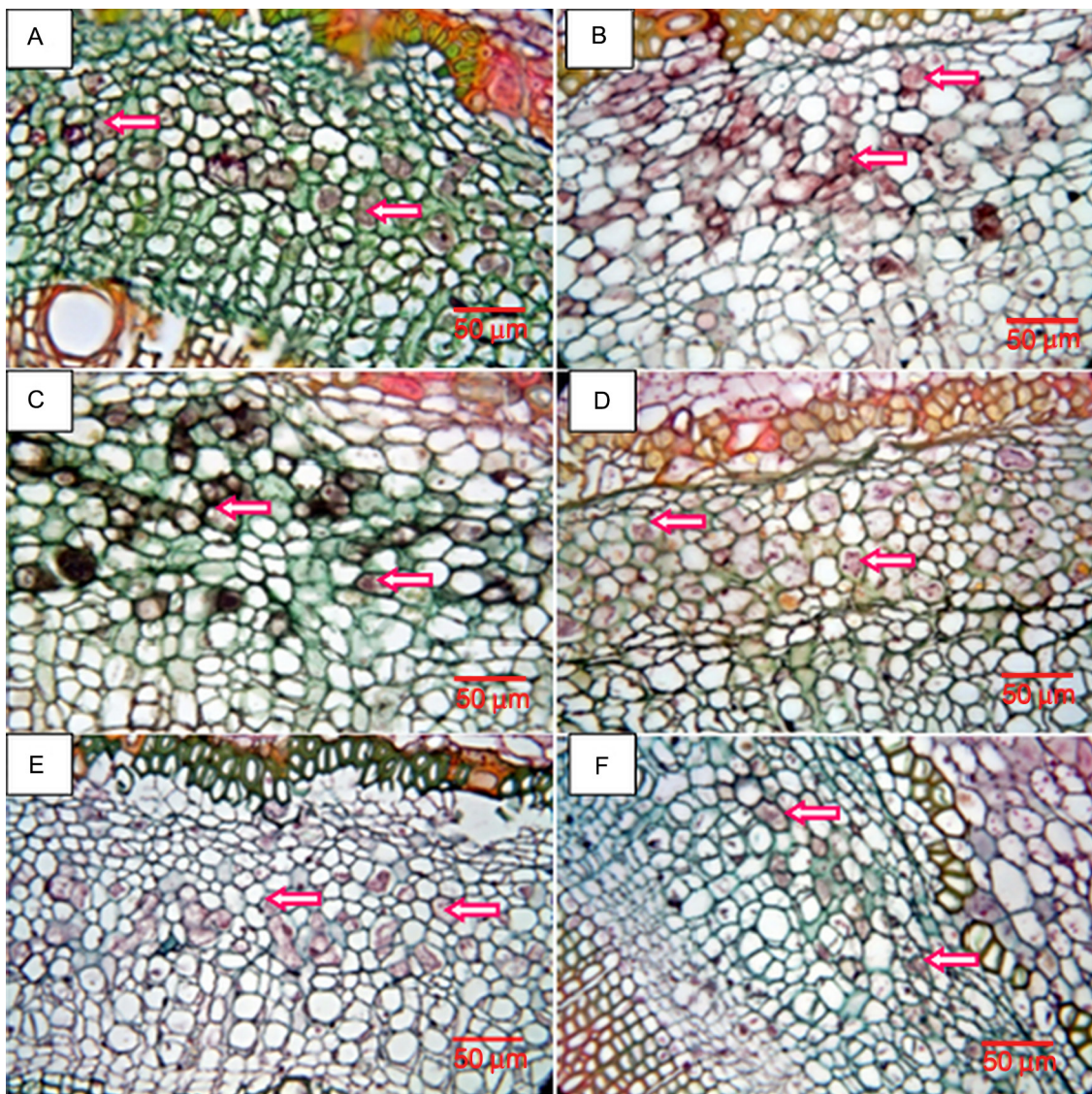
Figure 2 – Cross section of bark tissue of six Hevea brasiliensis clones A: SK1, B: SK3, C: NK1, D: T2, E: RRIT 251 and F: RRIM 600. The arrows indicate laticiferous cells. Bars = 50 \mu\text{m} .
