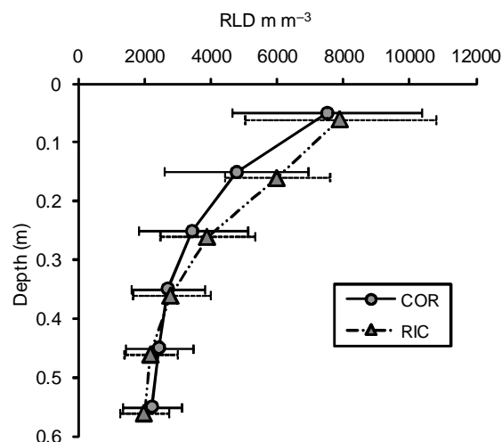
Figure 3 – Comparison of root length density profiles (RLD) obtained with the soil core sampling (COR) and root intersection counting (RIC) methods. Mean of 48 profiles (four dates 60, 170, 240, 280 DAR, and 12 replications).
