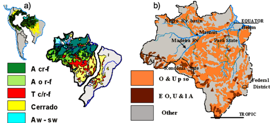
Figure 1 - (a) The original extent of the Brazilian Cerrado and main Amazon kind of vegetations: A c r-f = Amazon closed canopy rain-forest; A o r-f = Amazon open canopy rain-forest; T c/r-f = Transition cerrado/forest; Cerrado; & A w - s c = Amazon “white-sand campinarama” (mainly over Spodosols); (b) The agricultural and/or potentially arable soils within North and Central Brazil regions: O & U s u r = Oxisols and Ultisols (well drained and mostly on slight undulating or almost level relief phases 2 ); E A & U: Eutrophic soils (Eutrustox or Eutradox, Alfisols & some Ultisols). (Adapted from IBGE 1992 & 2004).
