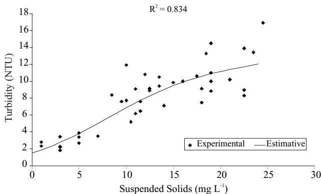
Figure 1 - Correlation between turbidity (Turb) and suspended solids (SS).
