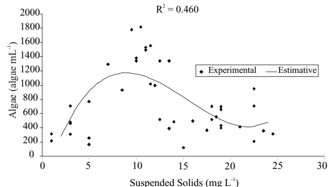
Figure 3 - Correlation between amount of algae (algae) and suspended solids (SS).
