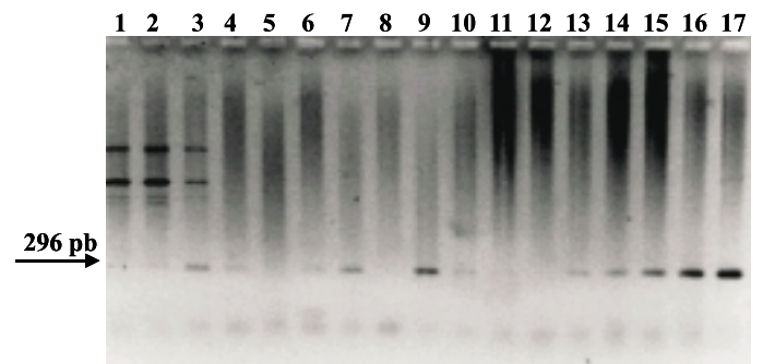
Fig. 3 - Electrophoresis in 2% agarose gel showing: in columns 12 to 17, amplicons with 296 bp of the plasmid titration (ten-fold dilutions; 17 = 8 \times 10^6 plasmids; 16 = 8 \times 10^5 plasmids; 15 = 8 \times 10^4 plasmids; 14 = 8 \times 10^3 plasmids; 13 = 8 \times 10^2 plasmids, and 12 = 80 plasmids. The amplicon band is not observed in column 12 due to the low plasmid quantity that is below the sensitivity of the test. Patient samples were run in columns 1 to 11, showing amplicon bands in columns 3 (15 768 CMV copies/ \mu g DNA); 7 (8 875 CMV copies/ \mu g DNA), and 9 (332 880 CMV copies DNA/ \mu g). In columns 1, 2, 4, 6 and 10, are shown amplicon bands with a lower density than the sensitivity of the test. In columns 5, 8 and 11, amplicon bands cannot be observed.
