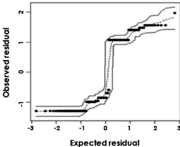
Figure 1 - The diagnosis of the logistic regression model. Since all residues are within the confidence band of the expected distribution, the model is well adjusted.
