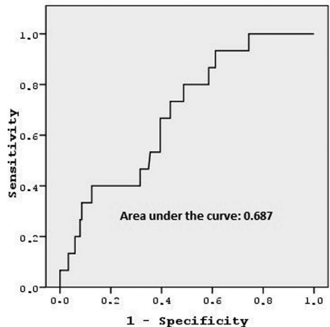
Figure 1 - ROC curve for NLR values.
