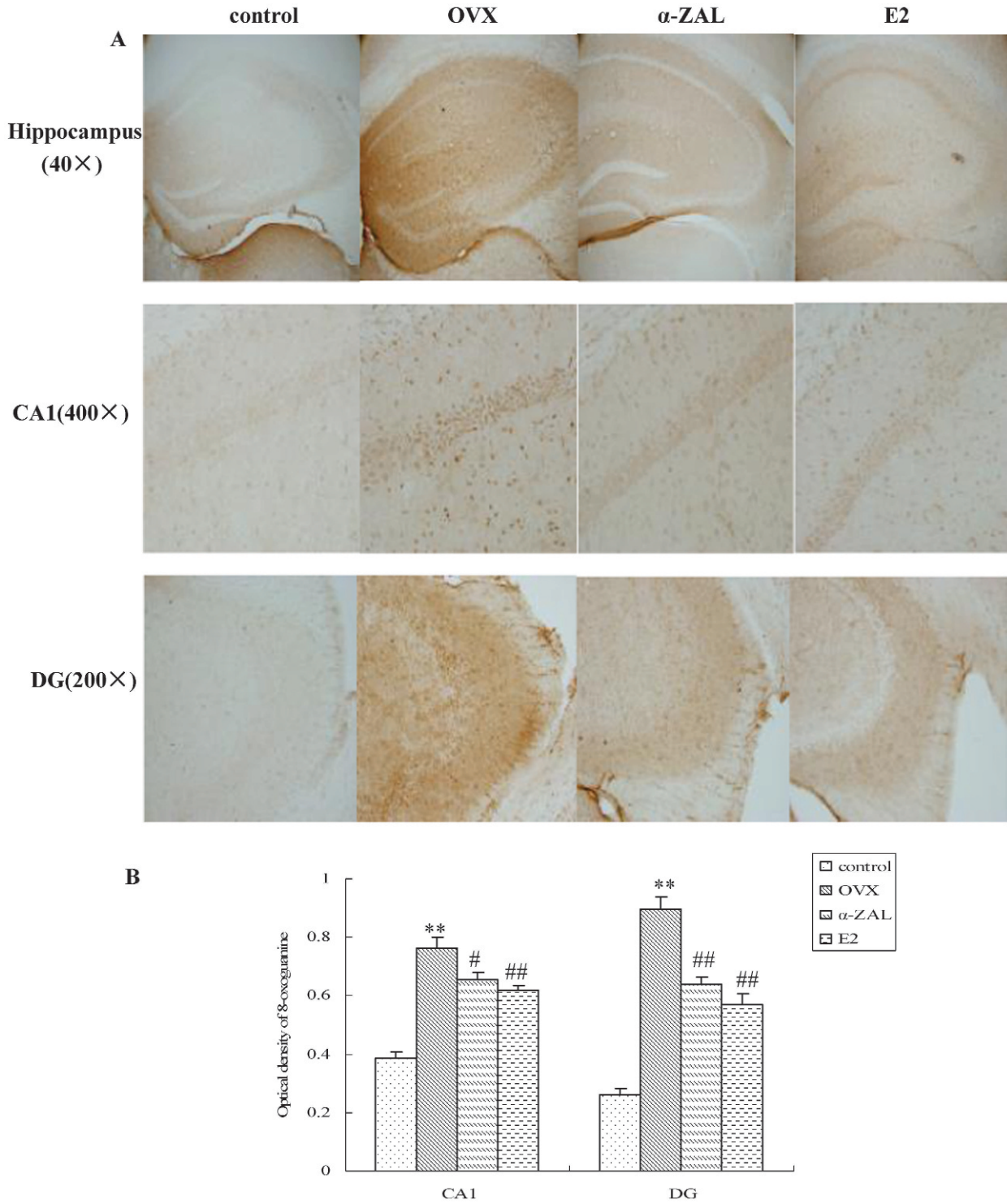
Figure 3 - The effect of E2 and \alpha -ZAL treatment on the levels of 8-oxoguanine in the hippocampi of mice. A. The immunohistochemical analyses of free-floating sections (25 \mu m in thickness). The first row shows a lower magnification of the hippocampus (40 \times ), whereas the magnified views of the CA1 (400 \times ) and DG (200 \times ) subregions are shown in the middle and last rows, respectively. B. Quantification of 8-oxoguanine immunolabeling in the CA1 and DG regions of the hippocampus. n = 4 in each group. The results represent at least three independent experiments in each animal. ** p < 0.01 vs. control group; # p < 0.05 and ## p < 0.01 vs. OVX group.
