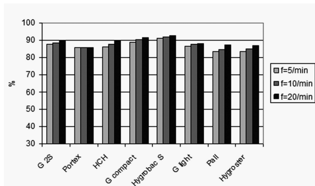
Figure 3 - Effect of respiratory frequency (5, 10 and 20/min) with changing %RAH. The %RAH did not depend on frequency. Again, differences in %RAH between HME were minimal.
