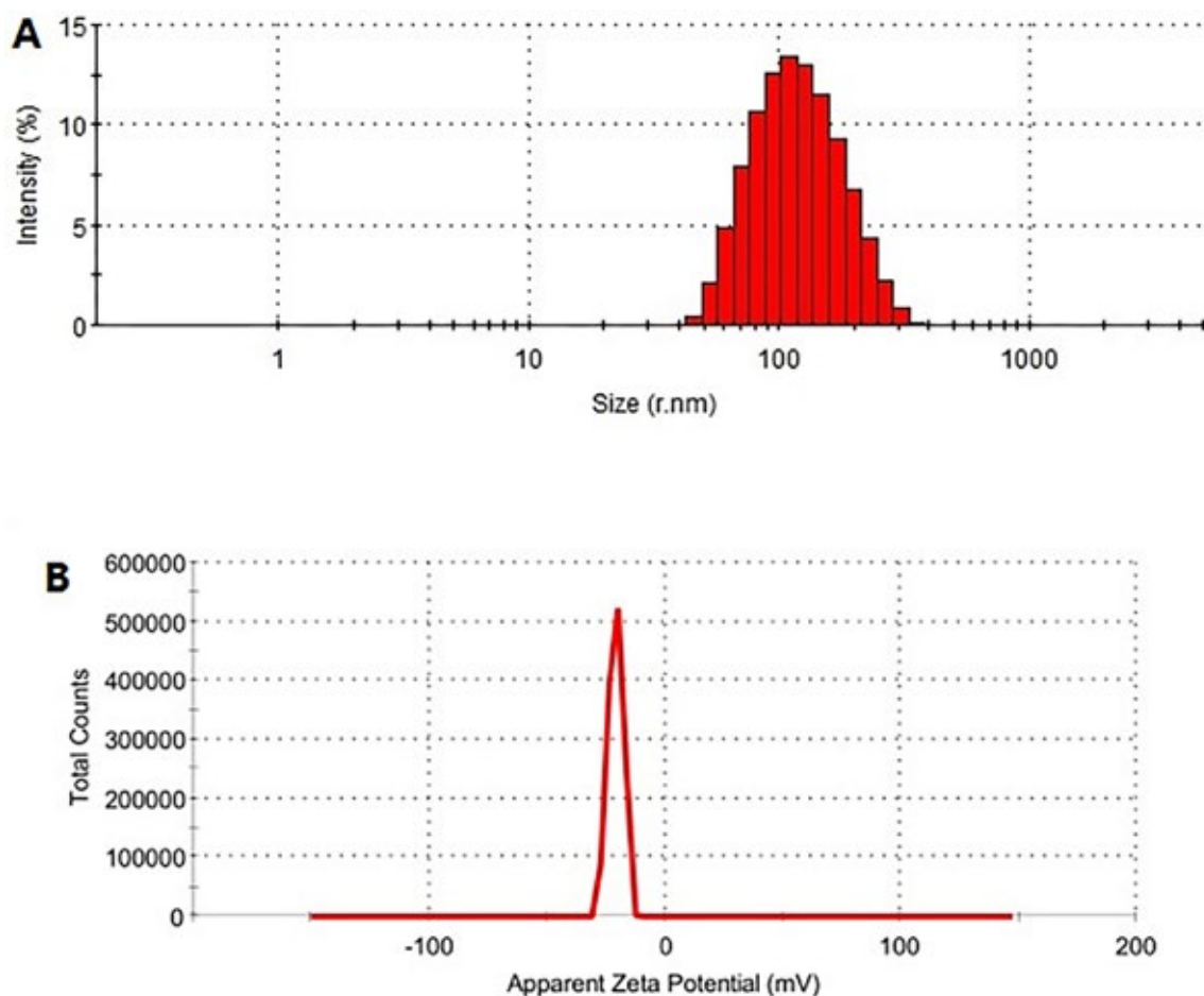
FIGURE 1 - Particle size and zeta potential of 2-ME-PSL.
