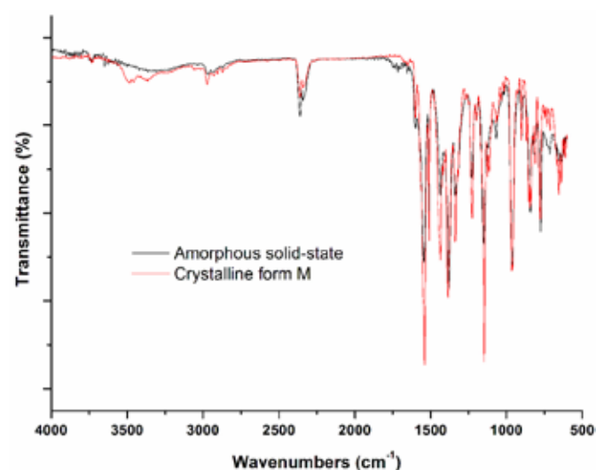
FIGURE 4 - IR spectra of ROSC in amorphous solid-state and crystalline form M.
