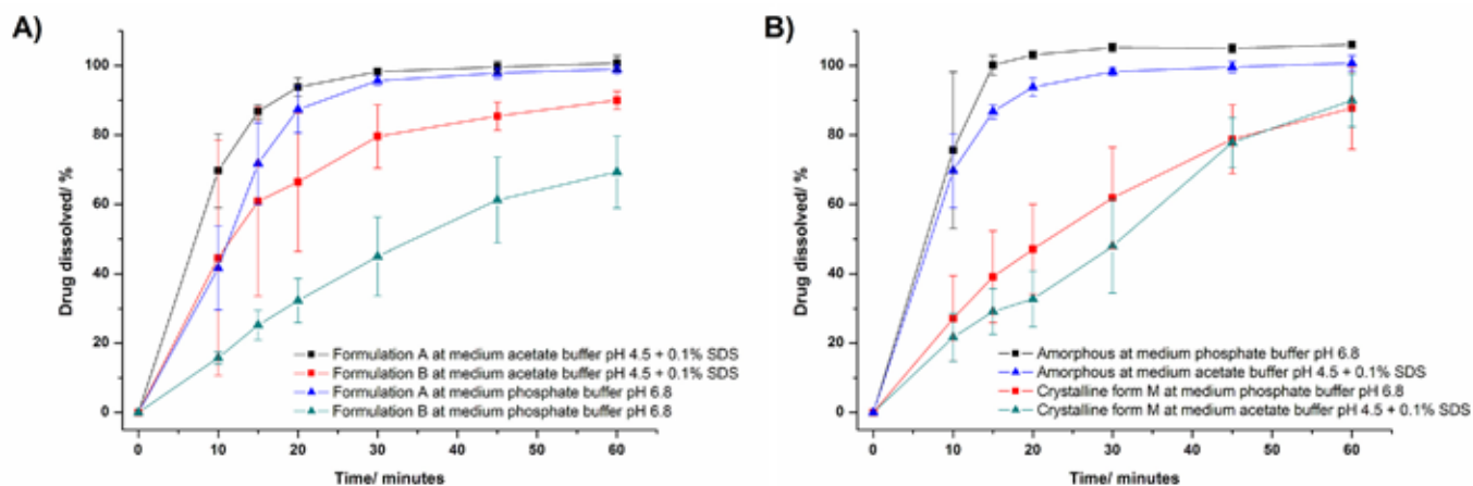
FIGURE 7 - Dissolution profiles of ROSC capsules from different media using basket at 100 rpm (n=6).
