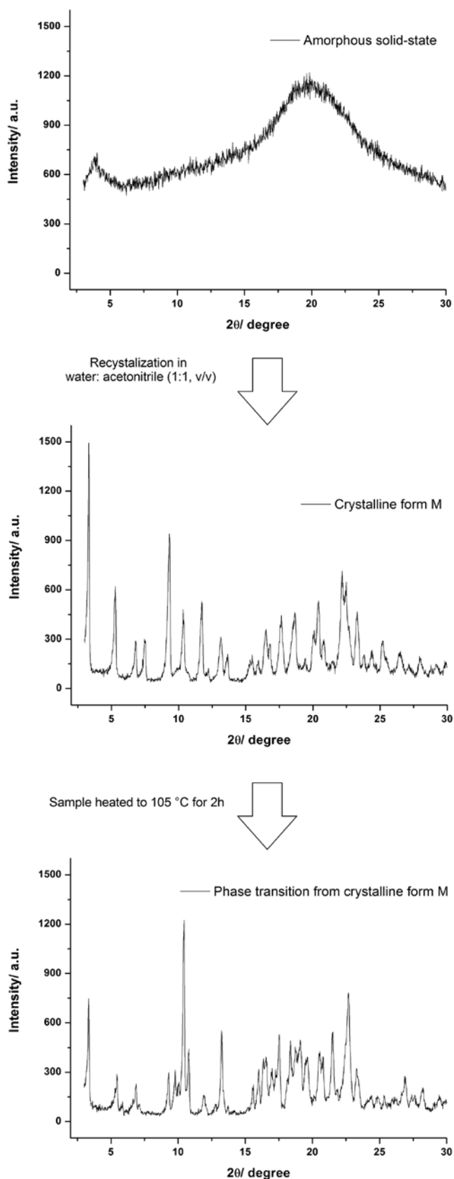
FIGURE 3 - XRD of ROSC: amorphous solid-state; crystalline form M, and its phase transition after heating to 105 °C for 2h.
