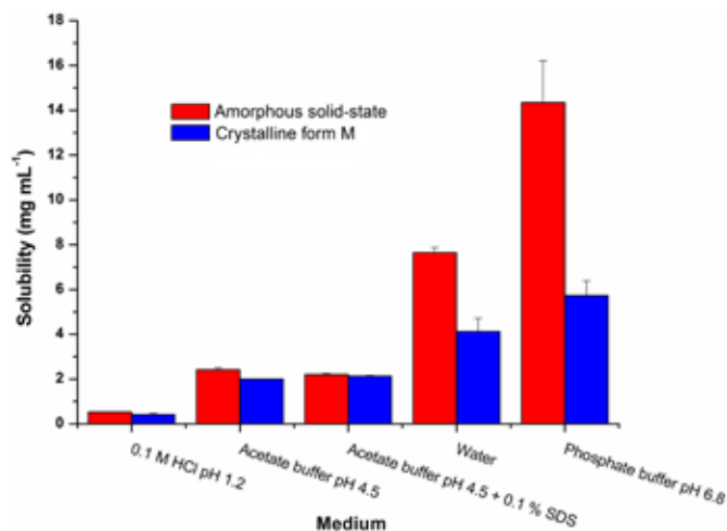
FIGURE 5 - Solubility of ROSC in aqueous media at 37°C (n=3).
