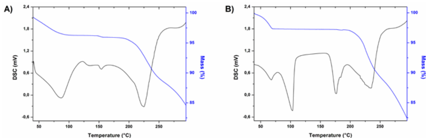
FIGURE 2 - DSC and TG curves of ROSC: A) Amorphous powder; B) Crystalline form M.
