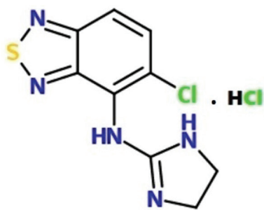
FIGURE 1 - Chemical structure of tizanidine HCl (MW = 290.17 Da, pKa = 7.4, Log p = 2.02, t_{1/2} = 2.25 hour).
