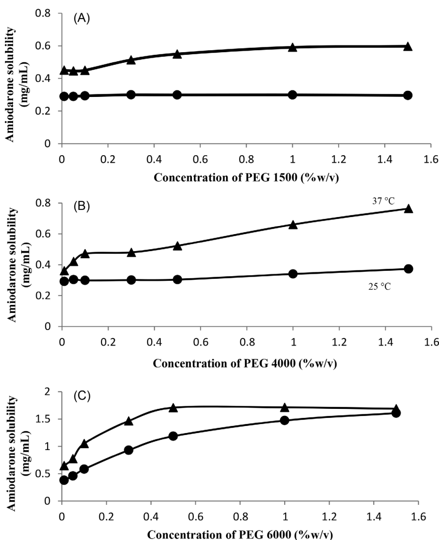
FIGURE 1 - Phase solubility curves of AMH in aqueous solutions of (A) PEG 1500, (B) PEG 4000 and (C) PEG 6000 at 25 and 37\text{ }^{\circ}\text{C} \pm 0.5\text{ }^{\circ}\text{C} ( n = 3 ).
