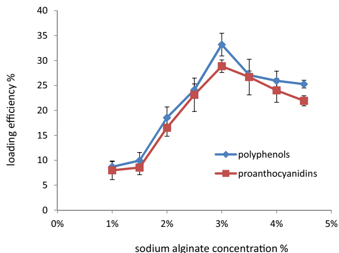
FIGURE 1 - Effect of sodium alginate concentration on total extractable polyphenols and proanthocyanidins loading efficiency. a Values are mean \pm SD, (n = 3).
