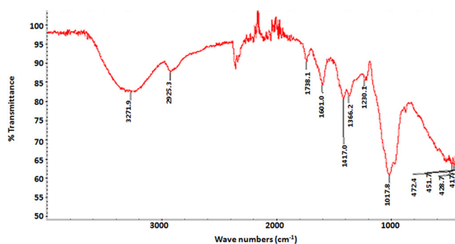
FIGURE 2 – FTIR spectrum Prunus domestica gum.
