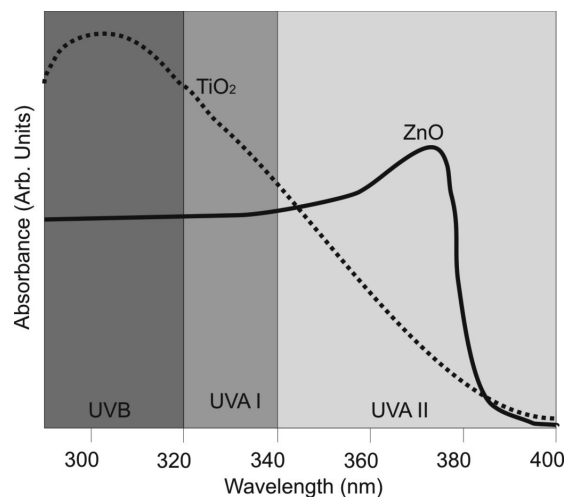
FIGURE 2 - Schematic demonstration of UVA and UVB absorbance by \text{TiO}_2 and ZnO UV filters.
