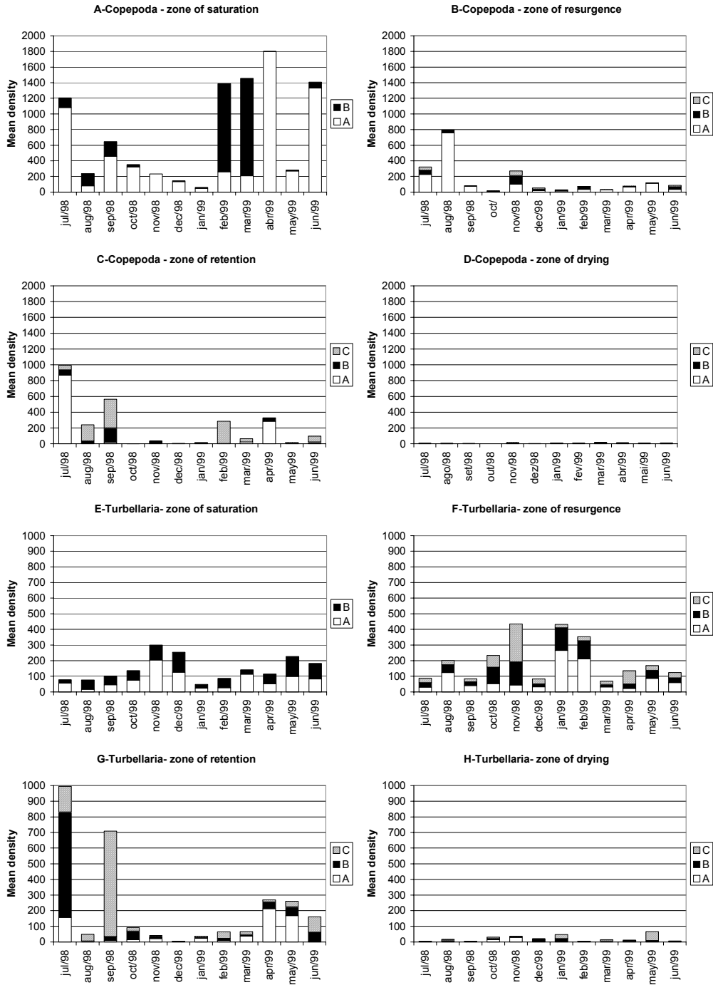
Fig. 5. Vertical distribution of Copepoda and Turbellaria during the sampling period. A=0-10 cm; B=10-20 cm; C=20-30 cm.
