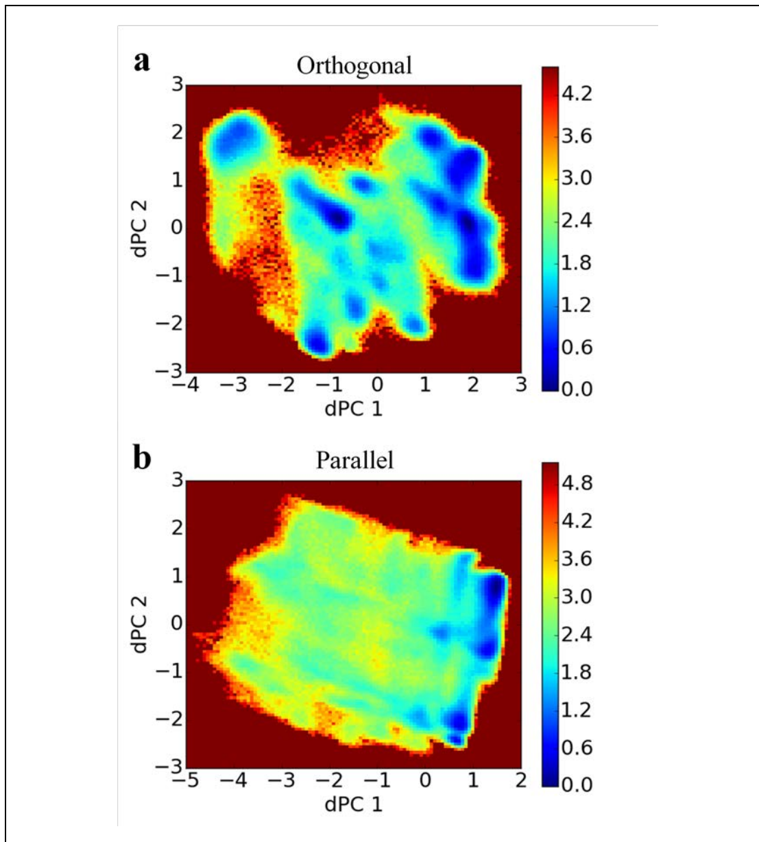
Figure 4.4. Free energy landscape of Aβ40 dimers. Energy landscapes are from 1.5 μs aggregate aMD simulations of Aβ40 in orthogonal (a) and parallel (b) configurations. Colorbar units are in k_B T .
