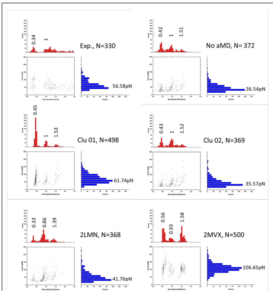
Figure 4.10. Experimental and MCP simulation results of force-induced dissociation of A \beta 40 dimers. Each dataset shows a scatter plot of Normalized Distance vs Force, a histogram of Force (blue), and a histogram of Normalized Distance (red); normalization was performed based on the experimentally observed contour lengths. Peak values, obtained using Gaussian distribution function, are presented above each peak of the histogram. Clu 01 and 02 are conformations from Figure 4.6 ; “No aMD” the most populated cluster before aMD simulations; and the bottom row are dimers from fibrils from the PDB. Statistical analysis was performed using two-sample Kolmogorov-Smirnov test with 0.05 significance level; only Clu 01 was statistically similar to the experimental data set, with p > 0.066 .
