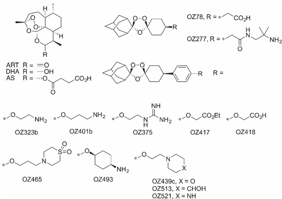
Fig. 1 Chemical structures of Ozonide Antimalarials and parent compounds artusunate (AS), artemisinin (ART), and dihydroartemisinin (DHA)
