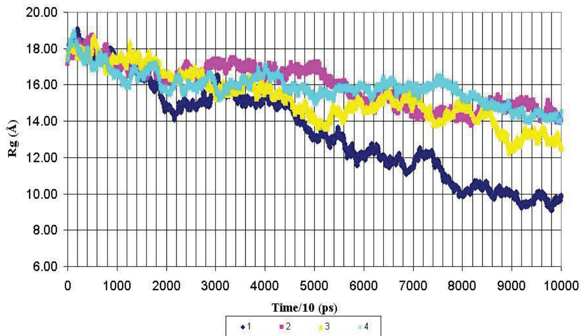
Figure 2. Radius of gyration ( R_g ) for backbone heavy atoms of the nonglycosylated peptide AHG21 – (1) and glycosylated peptides: AHG21 (T17) – (2), AHG21 (T5) – (3), AHG21 (T5, T17) – (4) during 1.0 ns MD simulations.
