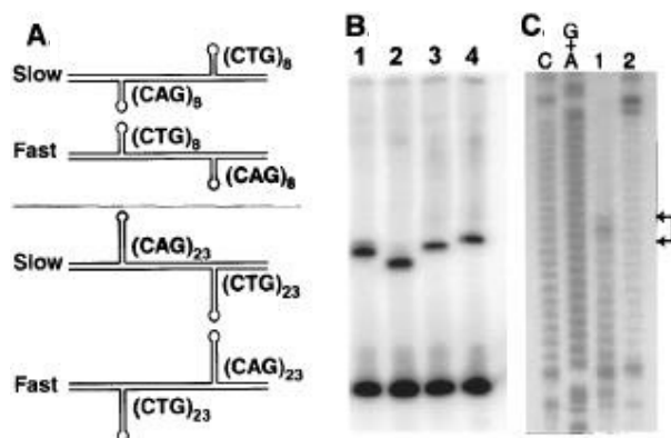
Figure 9. Properties of model slipped DNA constructs: effects of potential loop-loop interactions. (A) Different migration orders for heteroduplex isomers with short (non-interacting) and long (possibly interacting) triplet repeat loops. (B) The migration order for the long loops when the random sequences in two DNA strands cannot interact due to non-complementarity (lanes 1, 2) and when they are complementary (lanes 3, 4). Both pairs show 3' and 5' loop-outs in the top strand, respectively, as for the top pair of structures in A. (C) Chloroacetaldehyde reactivity of unpaired adenines and cytosines when the heteroduplex contains a single (CAG)_{23} loop (lane 1), and when it contains a complementary (CTG)_{23} loop 30 bp apart making an inter-loop interaction possible (lane 2).
