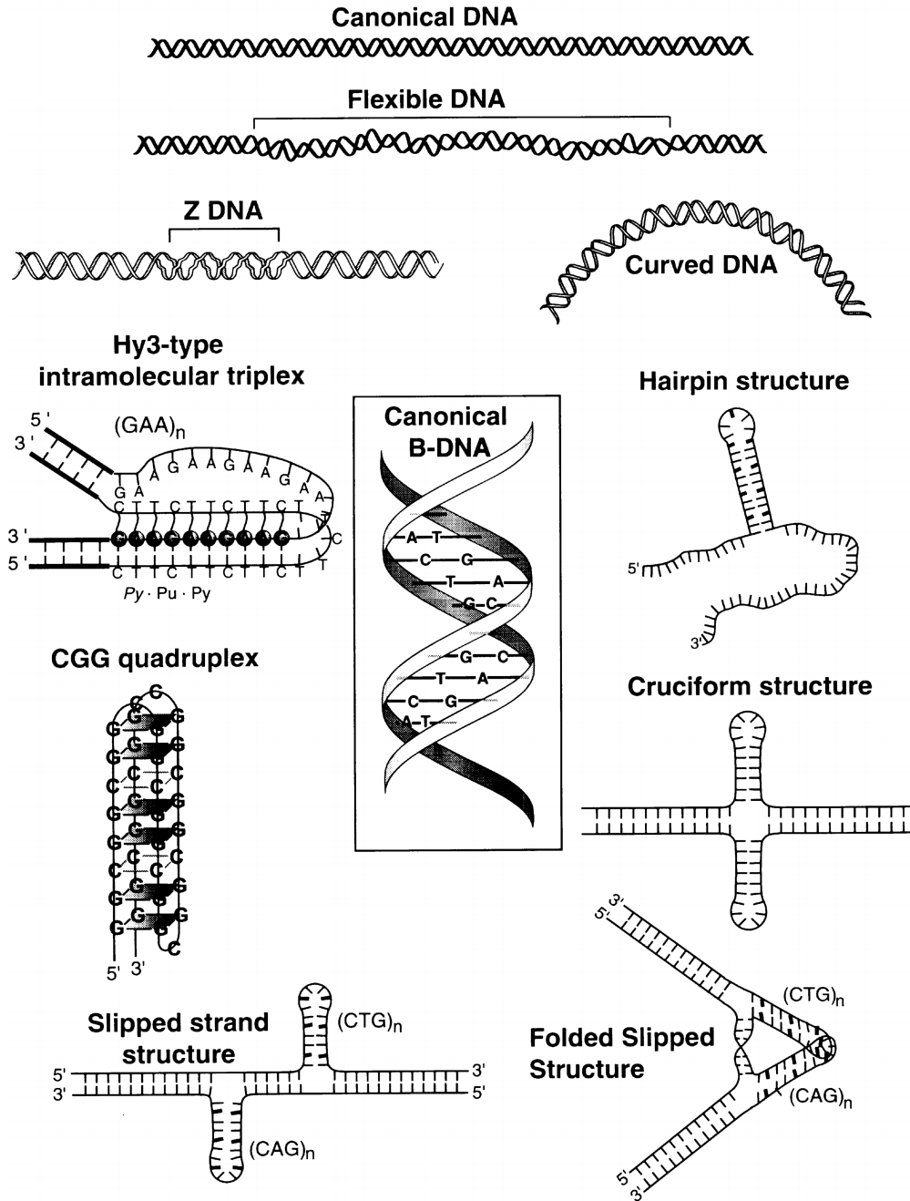
Figure 2. Alternative DNA structures formed in repeated DNAs. A canonical B-form helix is shown in a box in the center of the figure. A representation of this helix is also shown at the top of the figure. Although a straight molecule is shown, the DNA inherently possesses a certain degree of flexibility. (CTG)_n \bullet (CAG)_n and (CGG)_n \bullet (CCG)_n repeats, however, are extremely flexible compared to mixed sequence B-form DNA (shown below canonical DNA). The next two representations, Z-DNA and stable curved DNA, occur in (CG)_n \bullet (CG)_n and (GT)_n \bullet (AC)_n runs and DNA containing phased A_{4-5} \bullet T_{4-5} tracts (and other sequences), respectively, but have not been identified in triplet repeats. Proceeding clockwise, hairpin structures form in most disease-relevant triplet repeat single strands (to some degree). Cruciform structures form in perfect inverted repeats and have not been identified in triplet repeat sequences. Folded slipped strand structures and simple slipped strand structures form in (CTG)_n \bullet (CAG)_n and (CGG)_n \bullet (CCG)_n repeats, as discussed in the text. Quadruplex structures have been identified in oligonucleotides containing CGG and TGG repeats. In these structures the guanine are held together by G•G Hoogsteen bonds. A Hy3-type intramolecular triplex (as well as bi-triplex structures) can form in the (GAA)_n \bullet (TTC)_n repeat associated with Friedreich's ataxia.
