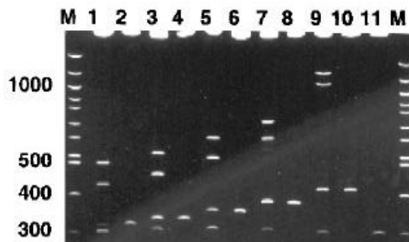
Figure 5. Electrophoretic separation in a polyacrylamide gel of 3-way junction heteroduplex isomers containing hairpins. This gel shows the separation of the hybridization products in a 5% native polyacrylamide gel. PvuII -digested plasmids with inserts in the EcoRI site were hybridized with PvuII -cut pUC8 and the products were separated in a polyacrylamide gel. The hybridization products contain 7 bp (lane 1), 12 bp (lane 3), 18 bp (lanes 5, 12), 27 bp (lane 7), and 50 bp (lane 9) hairpins. PvuII -digested insert-containing plasmids were included to identify the parental duplex fragments for the 7 bp- (lane 2), 12 bp- (lane 4), 18 bp- (lane 6), 27 bp- (lane 8), 50 bp-hairpin-containing fragments (lane 10), and pUC8 (lane 11), which contains no insert. Lanes M, 100 bp ladder molecular size markers. (This figure is modified from figure 2 from Oussatcheva et al 1999. Copyright, Academic Press.)
