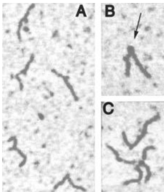
Figure 8. AFM images of (CTG)_{23} and (CAG)_{23} loop-outs. (A) Molecules with a single (CTG)_{23} loop-out. (B) A molecule with both a (CTG)_{23} and a (CAG)_{23} loop-out in opposite strands with 30 bp spacing. The two complementary loop-outs likely interact forming a bulky protrusion indicated by the arrow. (C) Representative dimer molecule, where interactions of complementary loops of the two double loop-out fragments stabilize the association of two molecules.
